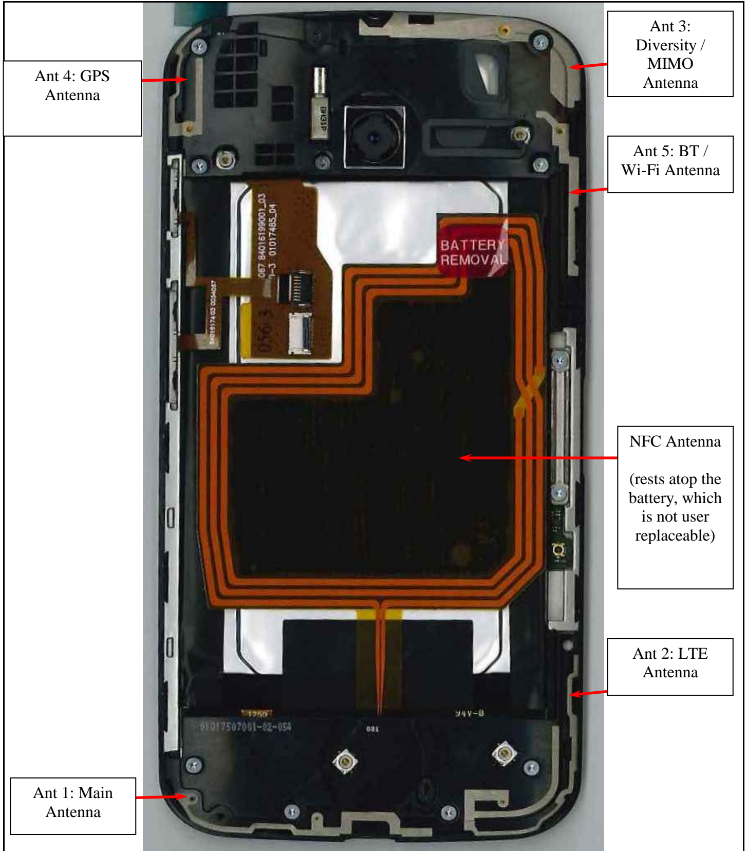
Photograph 9-4: Antenna Locations.
