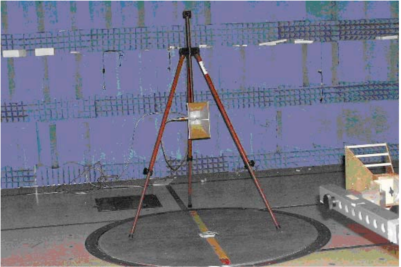
Figure 7c1-2: Antenna - Substitution.
