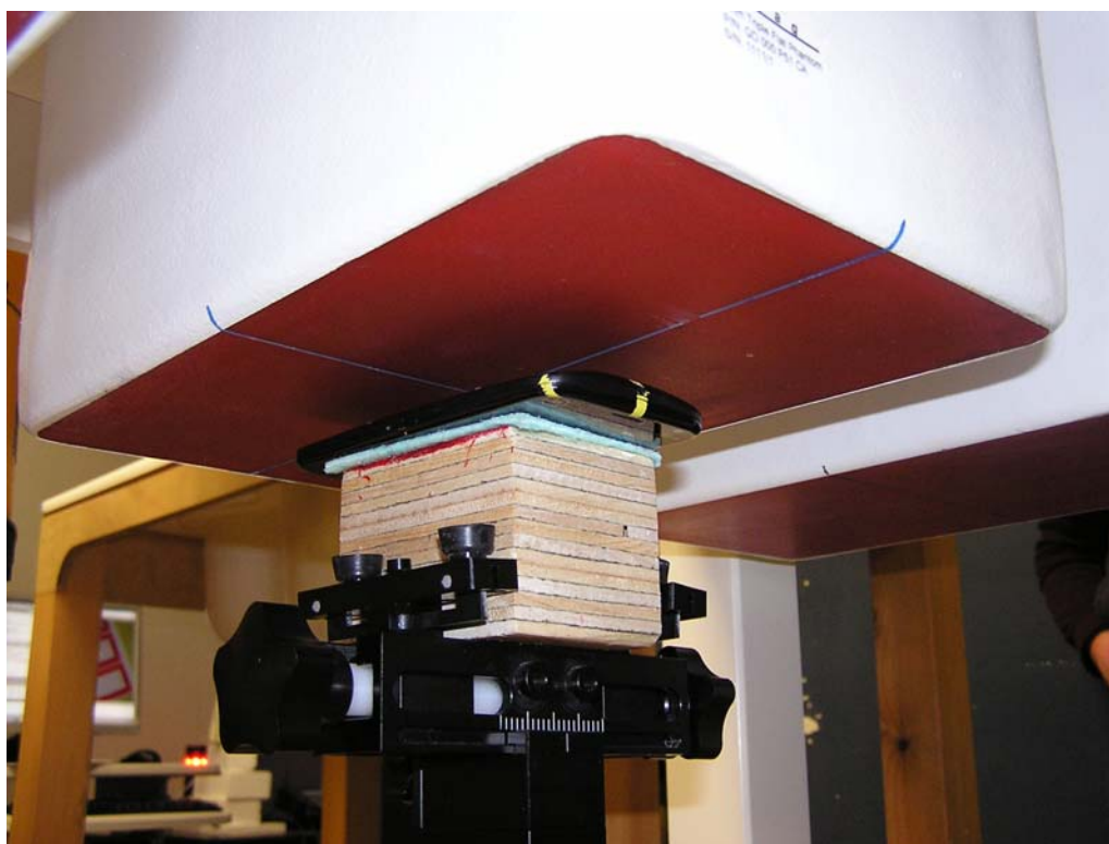
Figure 8: Mobile Hotspot Position, Back of Phone facing Phantom (10 mm separation)
