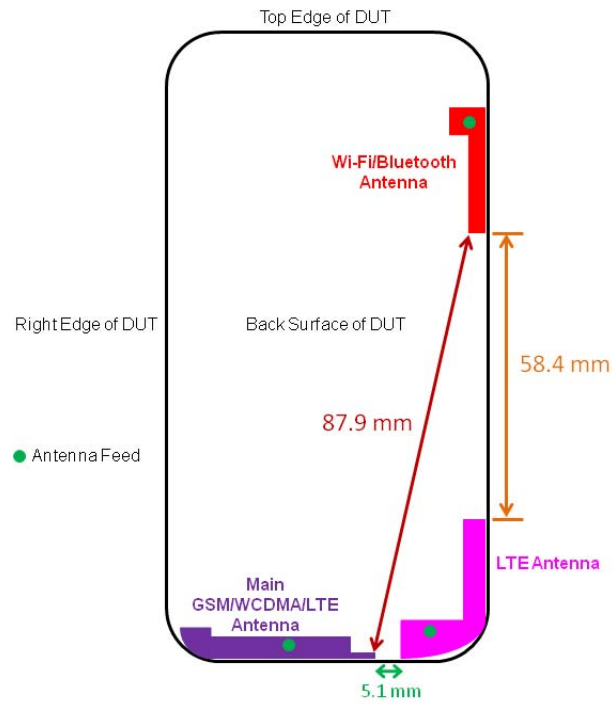
Figure 2: Antenna Locations and Separation Distances
