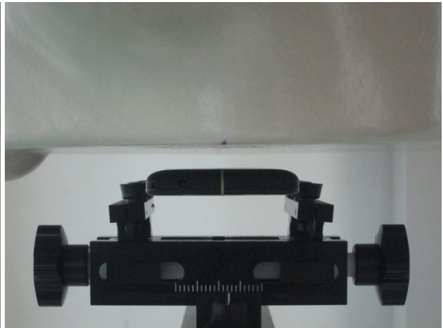
Back of the EUT with Phantom 1.0 cm Gap
