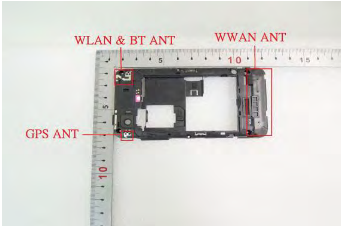
BT/ WLAN/ WWAN & GPS Antenna
