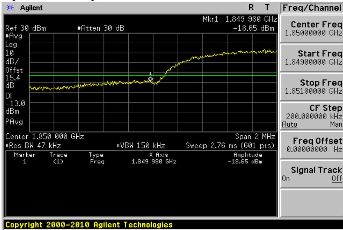
Figure 9-44: Band edge emission at antenna terminals –HSDPA II Channel Lowest
