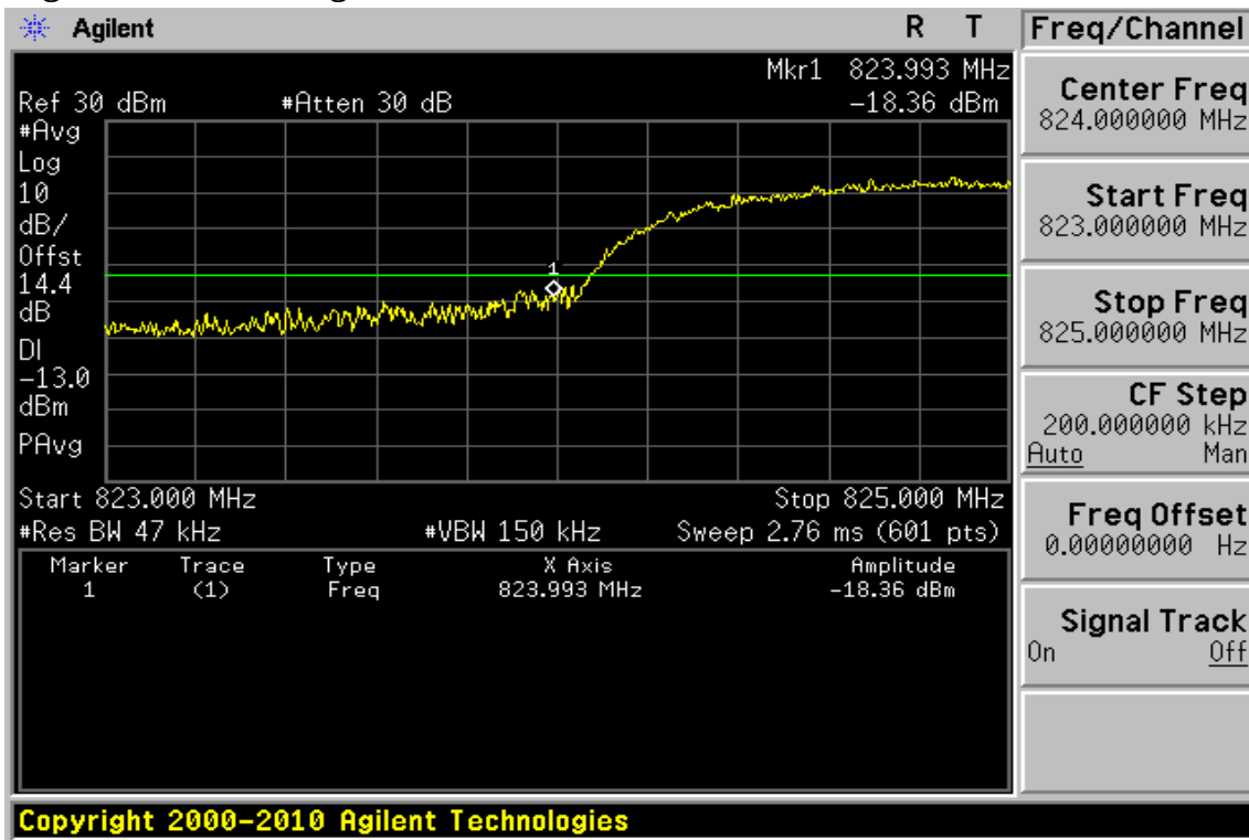
Figure 9-49: Band edge emission at antenna terminals –HSDPA V Channel Lowest
