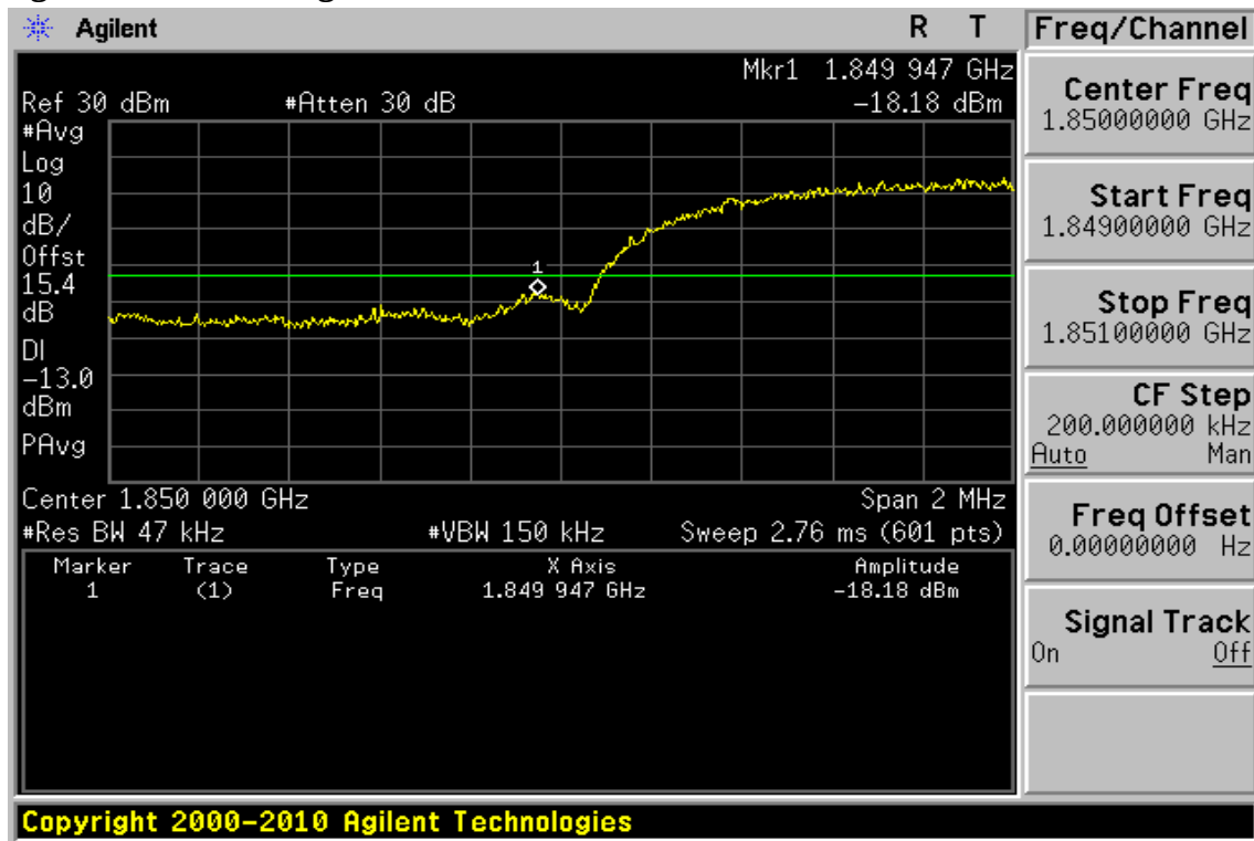
Figure 9-24: Band edge emission at antenna terminals –WCDMA II Channel Lowest
