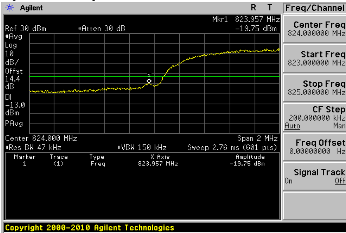
Figure 9-39: Band edge emission at antenna terminals –HSUPA V Channel Lowest
