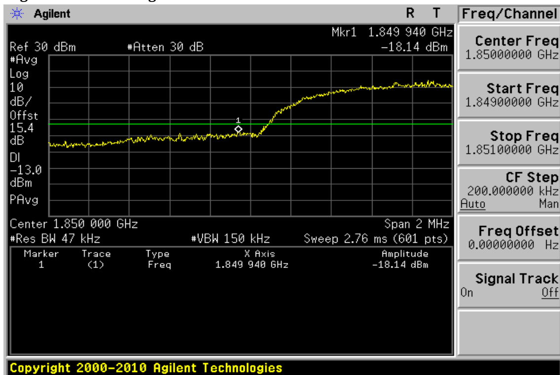
Figure 9-34: Band edge emission at antenna terminals –HSUPA II Channel Lowest
