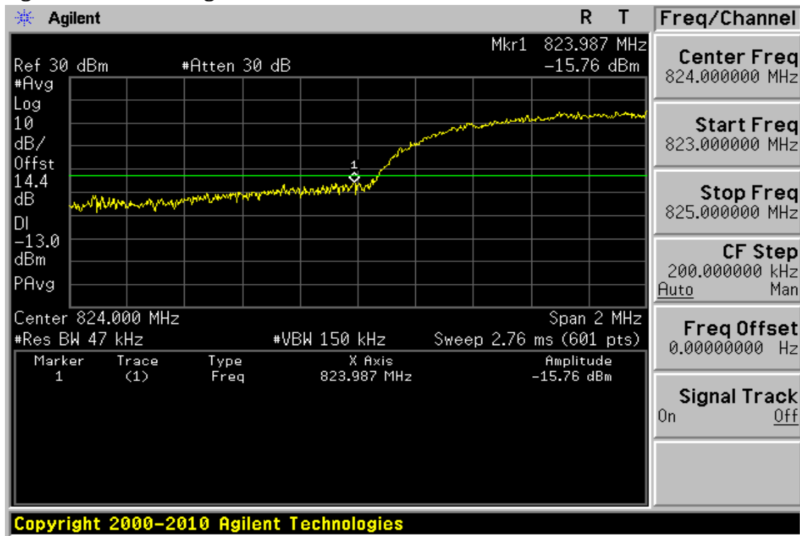
Figure 9-29: Band edge emission at antenna terminals –WCDMA V Channel Lowest
