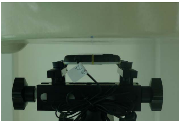
Back of the DUT with Phantom 1.5 cm Gap (Headset)
