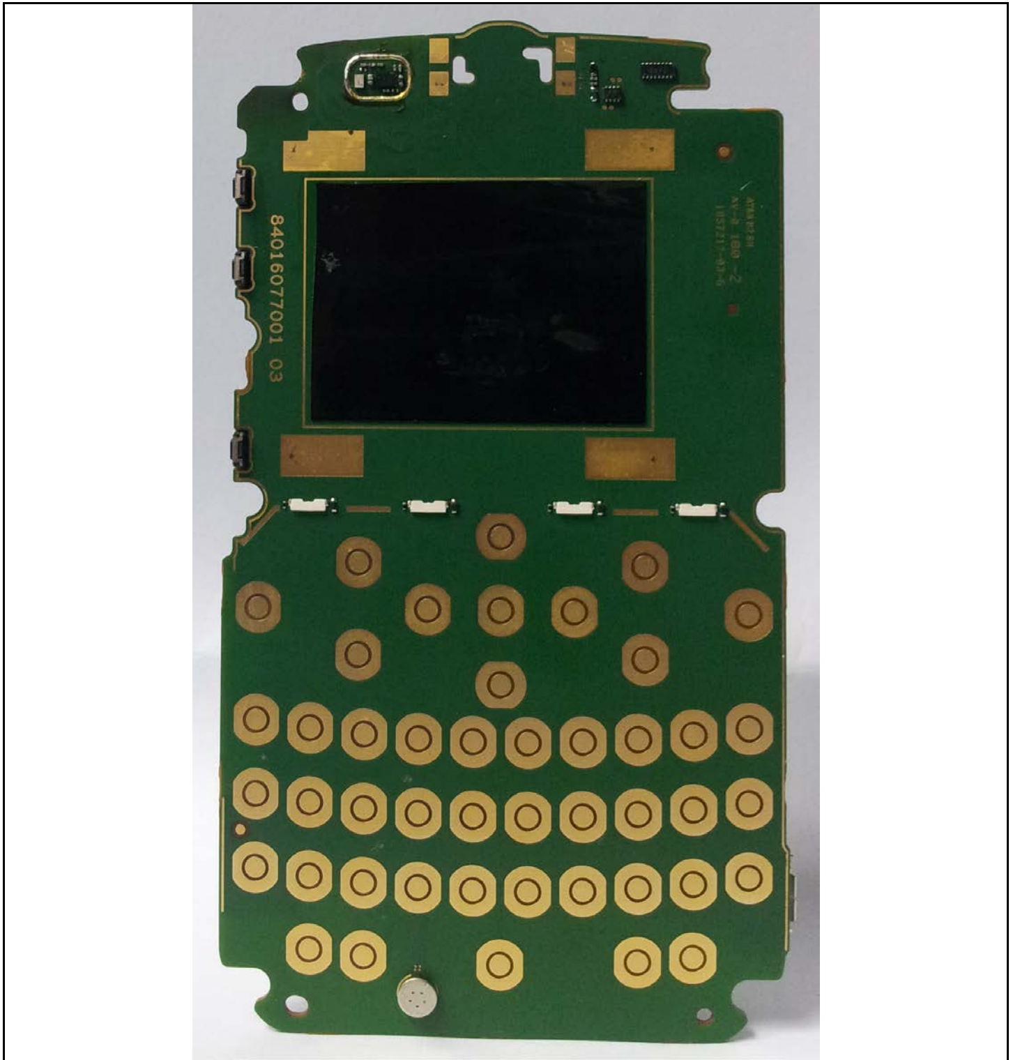
Photograph 9-2: Front side view of the device's PC Board, Shields Removed.
