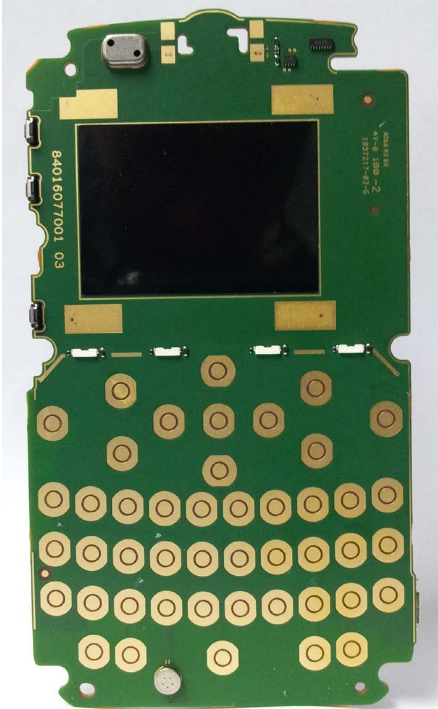
Photograph 9-1: Front side view of the device's PC Board, Shields in Place.
