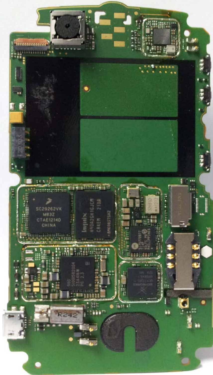
Photograph 9-4: Back side view of the device's PC Board, Shields Removed.
