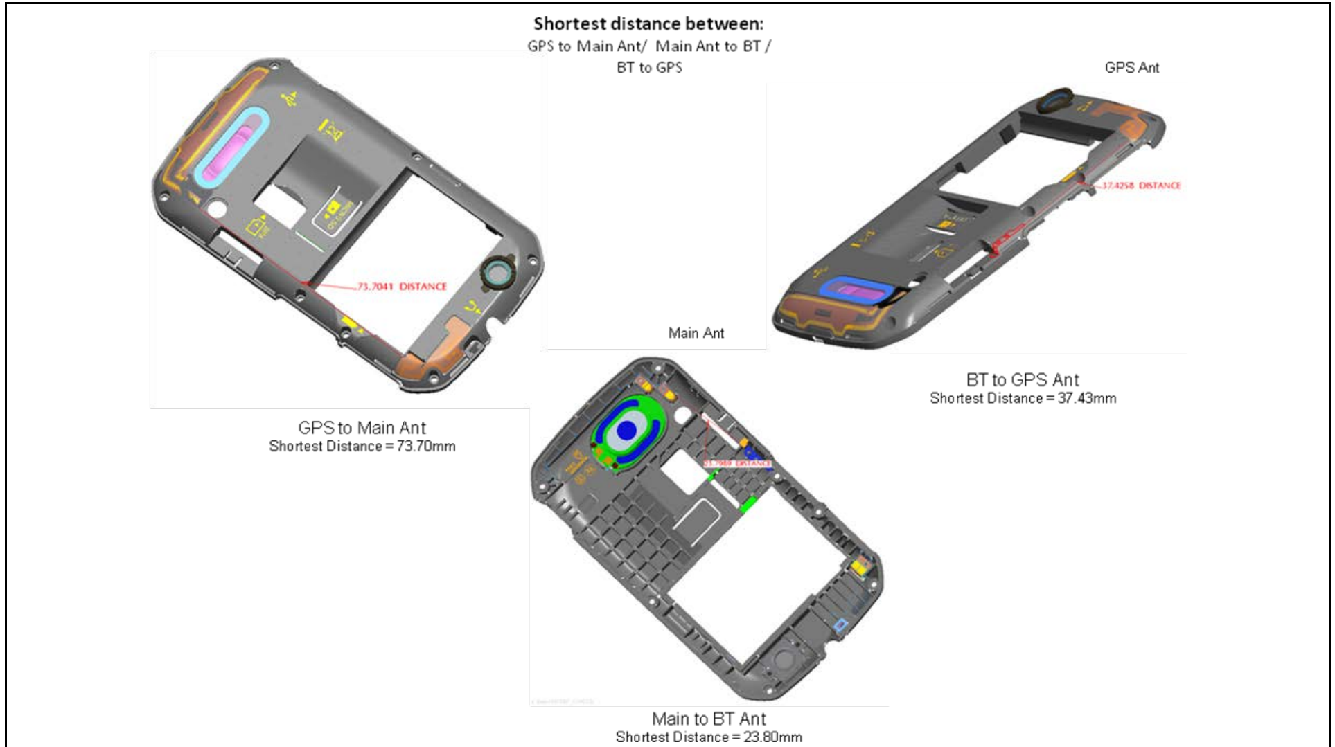
Photograph 9-5: Antenna Locations and Spacings.
