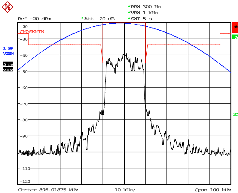
Figure 6a-2.2.1. iDEN 900 MHz Band, QPSK, Maximum Power, Emission Mask G
