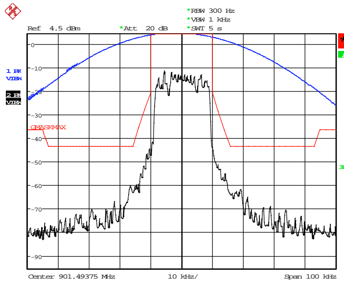
Figure 6b.2.1-1 iDEN NBPCS Band, Occupied Bandwidth, QPSK, Max.Power.
