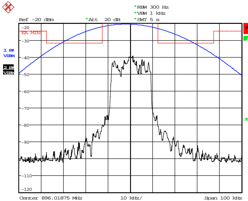
Figure 6a-2.2.3. iDEN 900 MHz Band, QPSK, Maximum Power, EA Emission Mask
