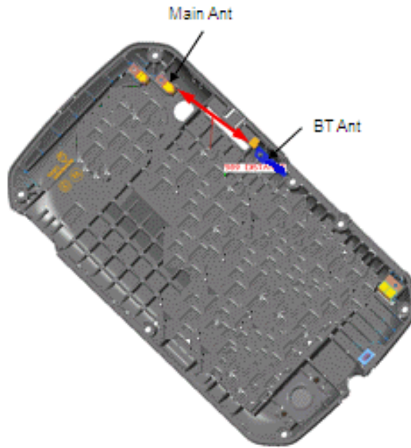
Figure 3: Antenna Separation Distances
