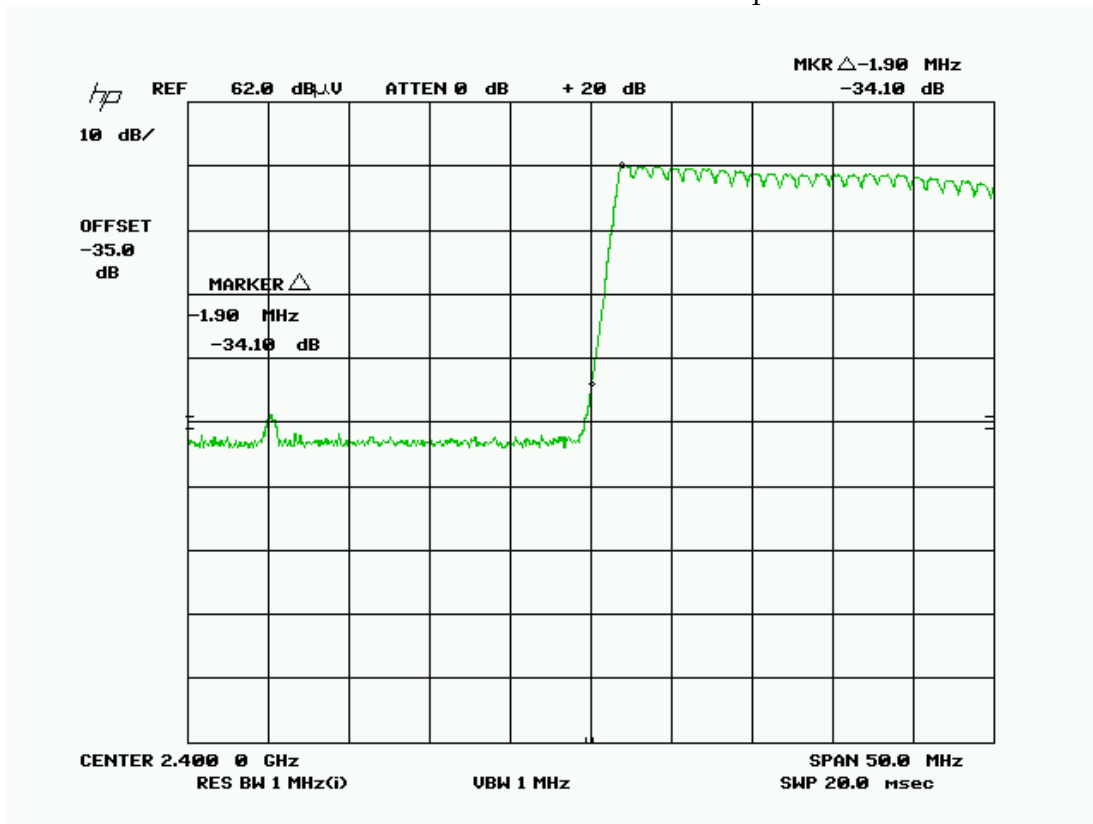
ch 2412-Lower restricted band peak
