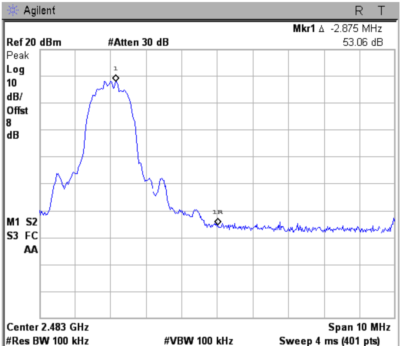
Figure 6d.6-10: Plot of upper band-edge conducted emissions with hopping disabled (8 DPSK Modulation).
