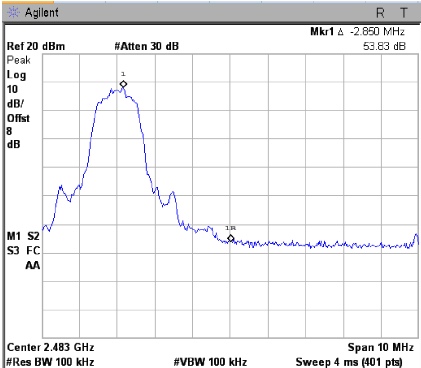
Figure 6d.6-6: Plot of upper band-edge conducted emissions with hopping disabled (Pi/4 DPSK Modulation).
