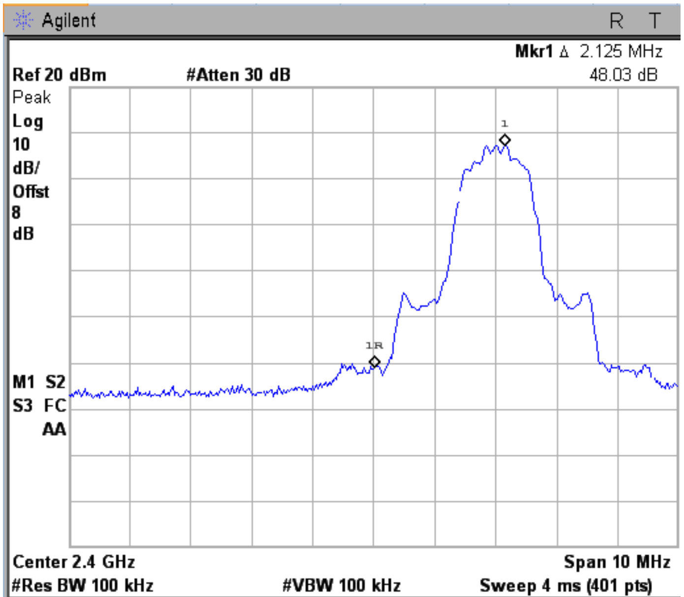
Figure 6d.6-5: Plot of lower band-edge conducted emissions with hopping disabled (Pi/4 DPSK Modulation).
