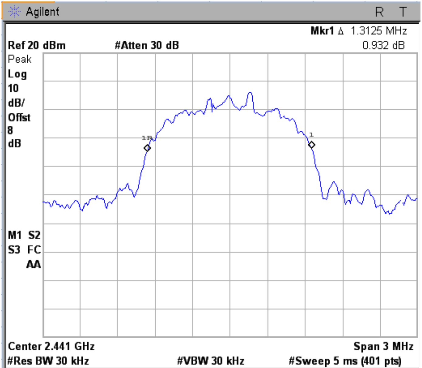
Figure 6d.2-3: Plot of 20 dB bandwidth (8-DPSK Modulation)
