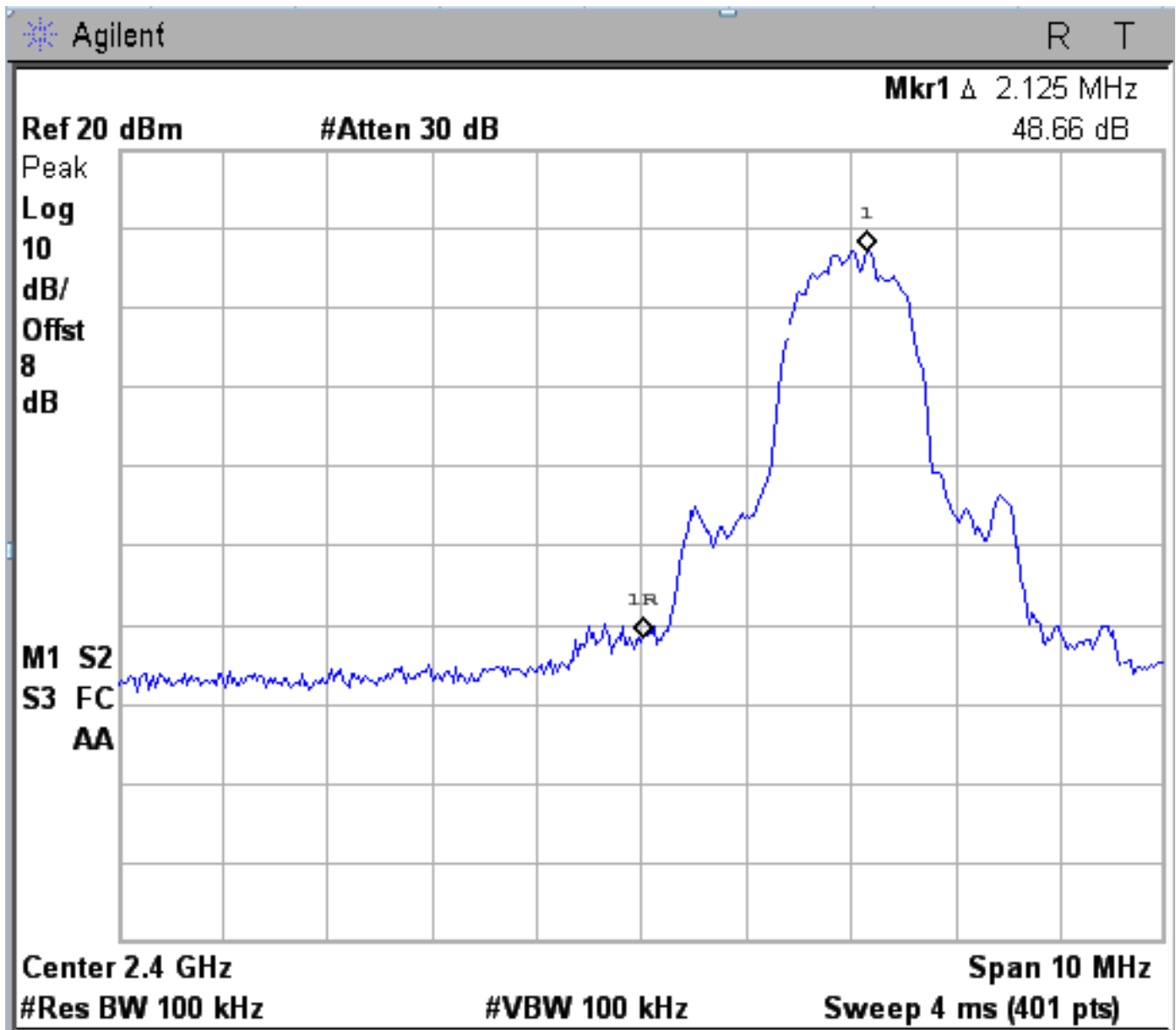
Figure 6d.6-9: Plot of lower band-edge conducted emissions with hopping disabled (8 DPSK Modulation).
