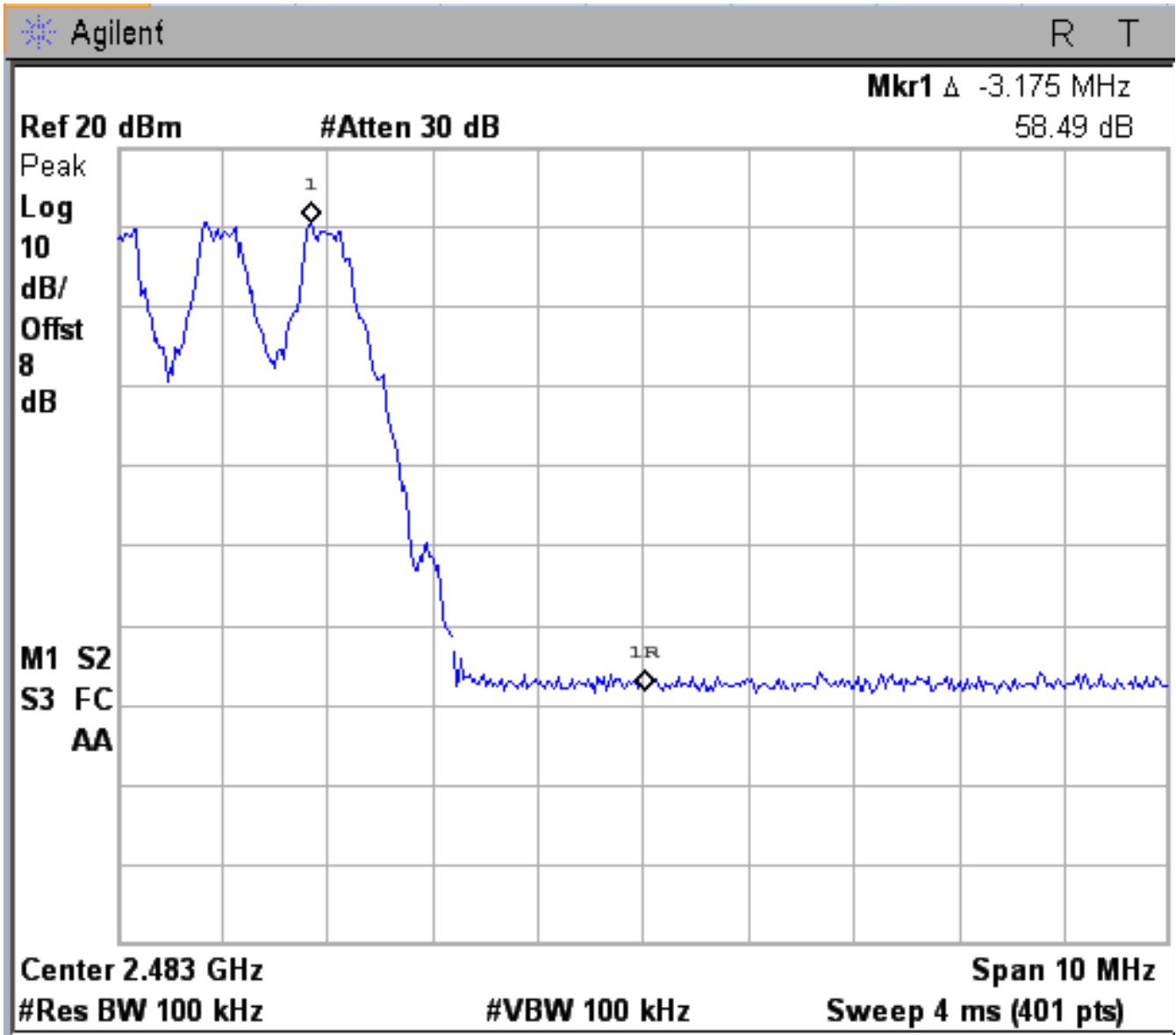
Figure 6d.6-4: Plot of upper band-edge conducted emissions with hopping enabled (GFSK Modulation).
