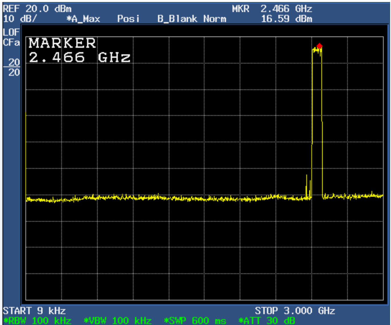
Figure 6d.7-10: Plot of spurious conducted emissions 9.0 kHz – 3.0 GHz (Hopping enabled).
