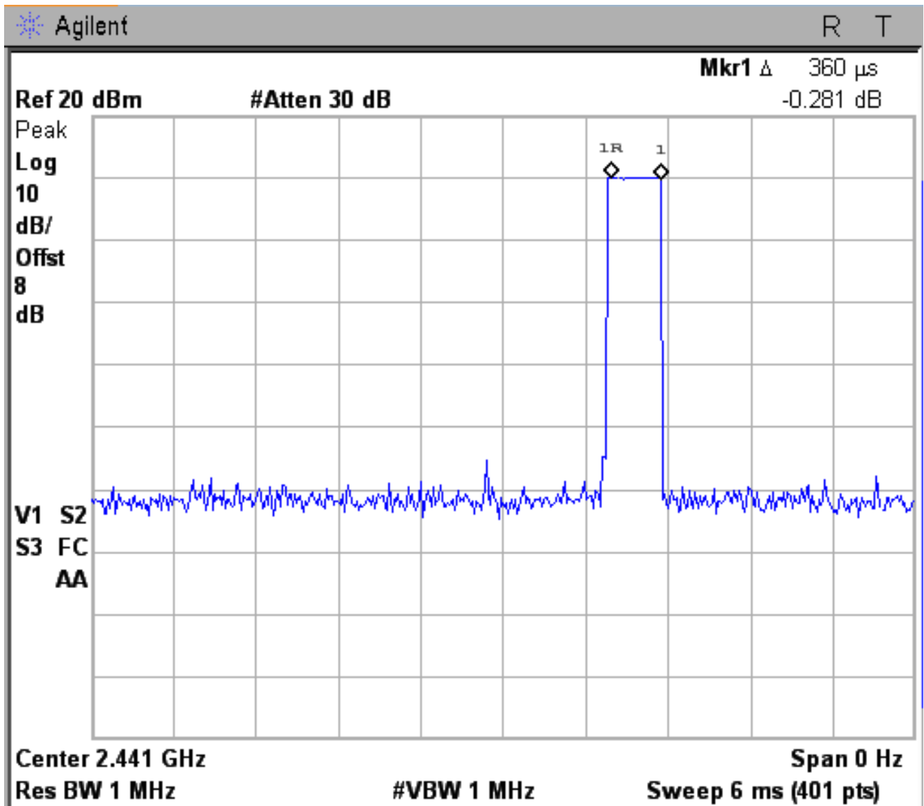
Figure 6d.4-4: Plot of dwell time over 6 ms period.
