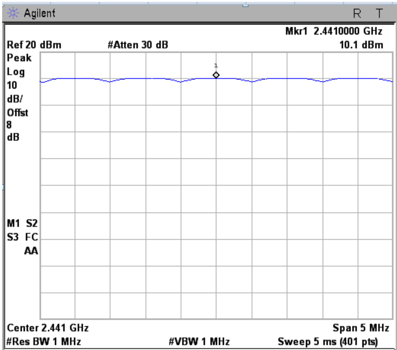
Figure 6d.5-1: Plot of peak output power
