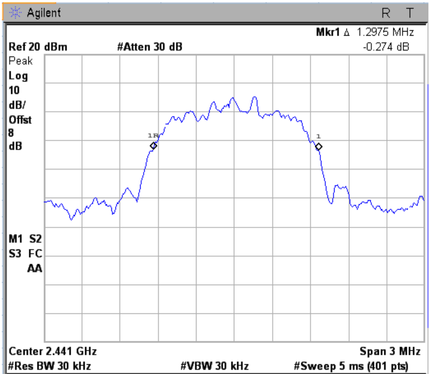
Figure 6d.2-2: Plot of 20 dB bandwidth (Pi/4 DPSK Modulation)
