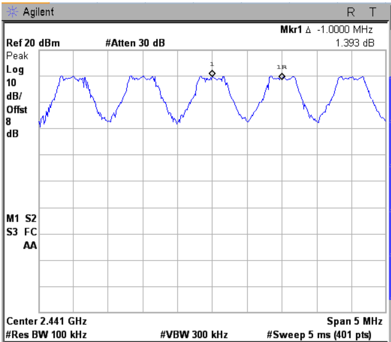
Figure 6d.1-1: Plot of Bluetooth carrier frequency separation
