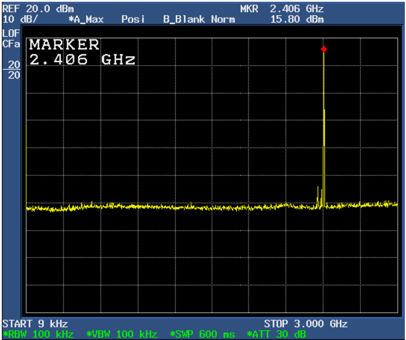
Figure 6d.7-1: Plot of spurious conducted emissions 9.0 kHz – 3.0 GHz (Low channel enabled).
