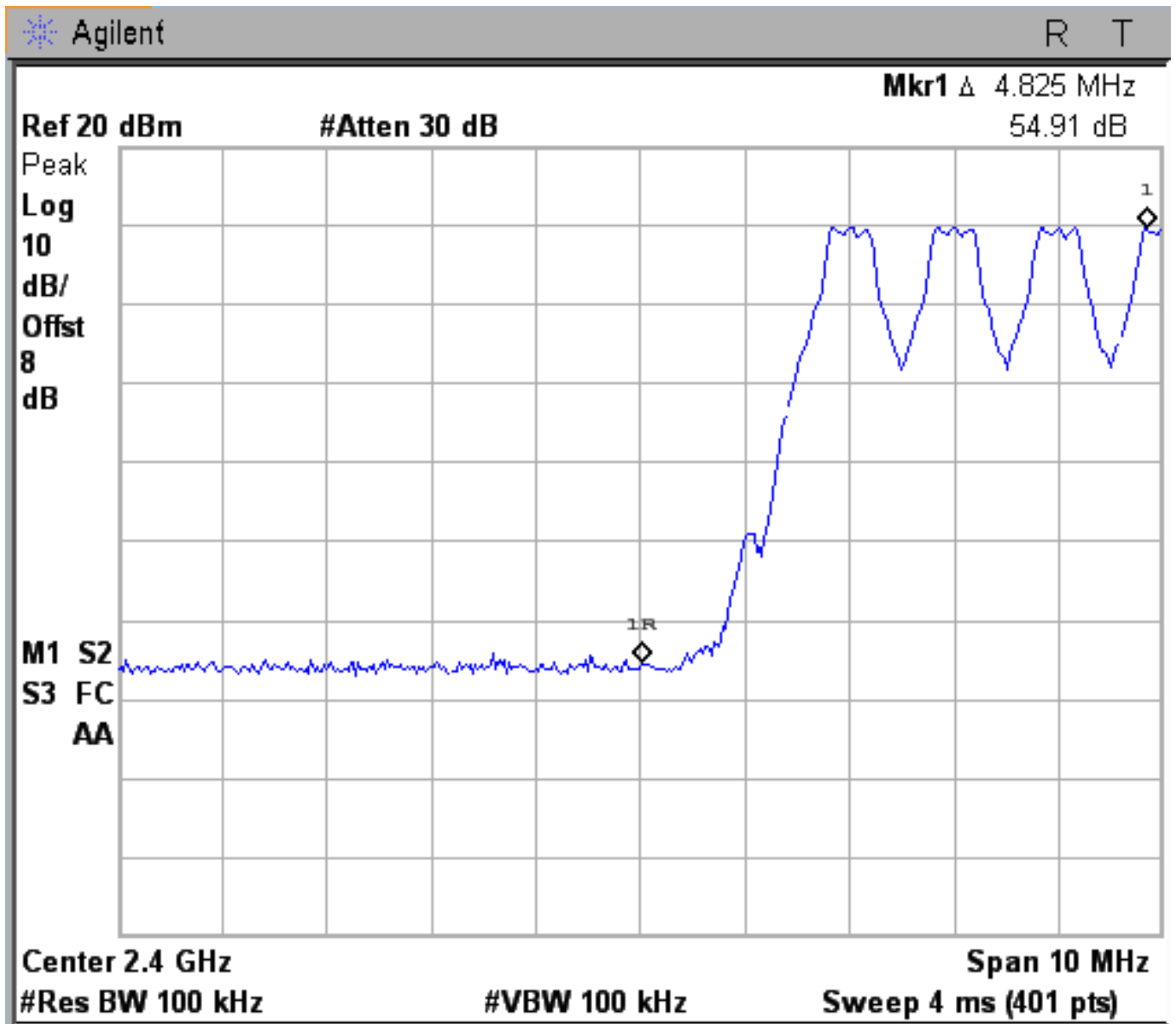
Figure 6d.6-3: Plot of lower band-edge conducted emissions with hopping enabled (GFSK Modulation).
