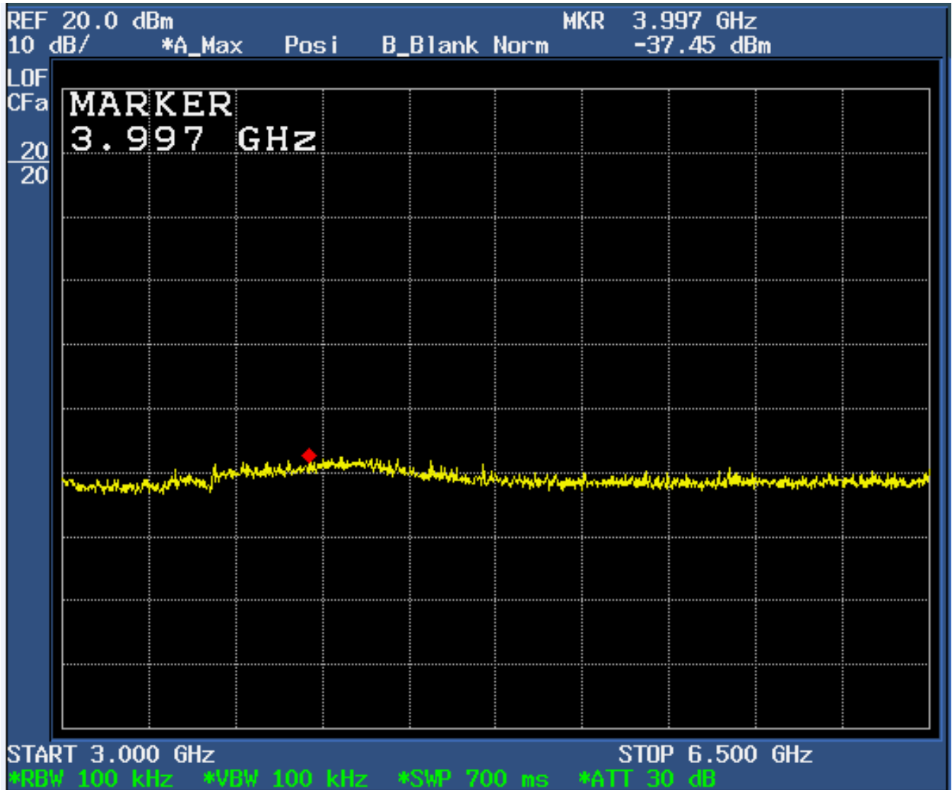
Figure 6d.7-11: Plot of spurious conducted emissions 3 GHz – 6.5 GHz (Hopping enabled).
