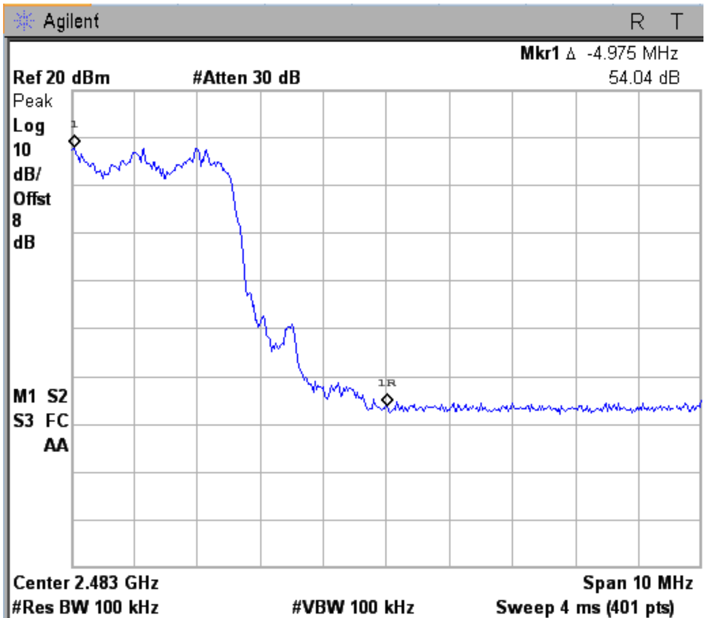
Figure 6d.6-8: Plot of upper band-edge conducted emissions with hopping enabled (Pi/4 DPSK Modulation).
