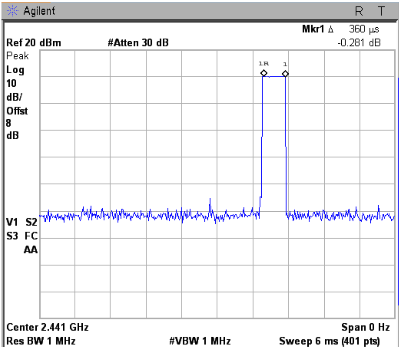
Figure 6d.4-3: Plot of dwell time over 6 ms period.
