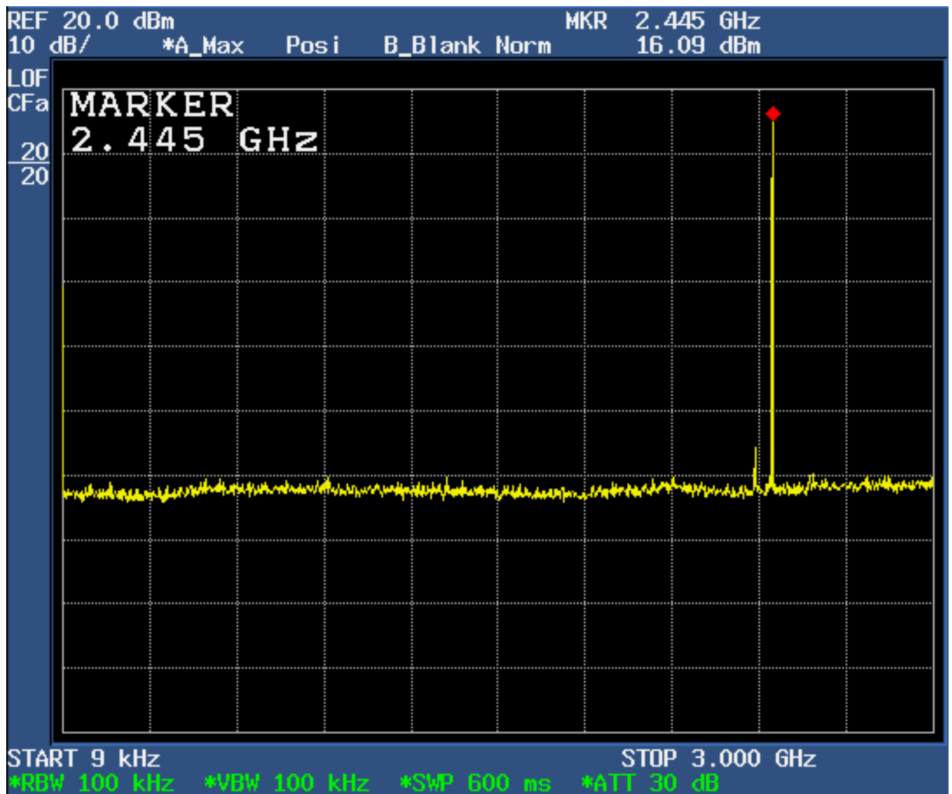
Figure 6d.7-4: Plot of spurious conducted emissions 9.0 kHz – 3.0 GHz (Mid channel enabled).
