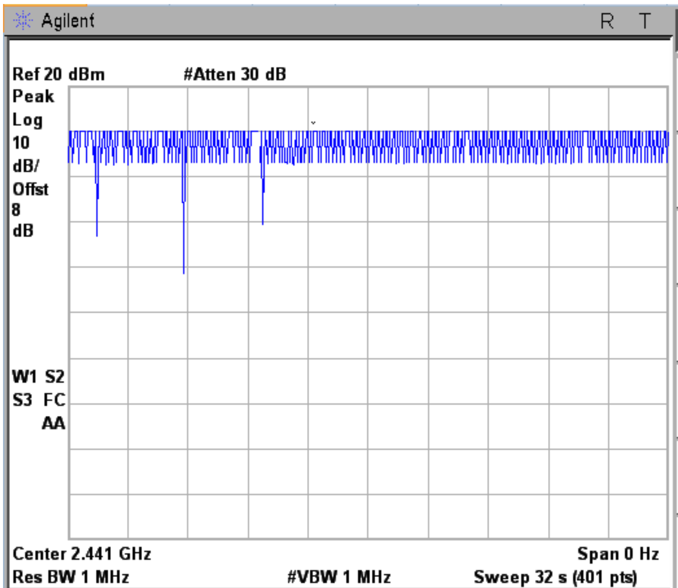
Figure 6d.4-1: Plot of dwell time over 32-second period
