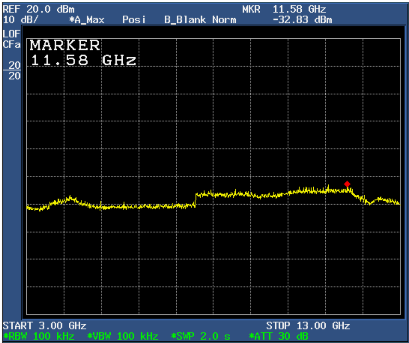
Figure 6d.7-8: Plot of spurious conducted emissions 3 GHz – 13 GHz (High channel enabled).
