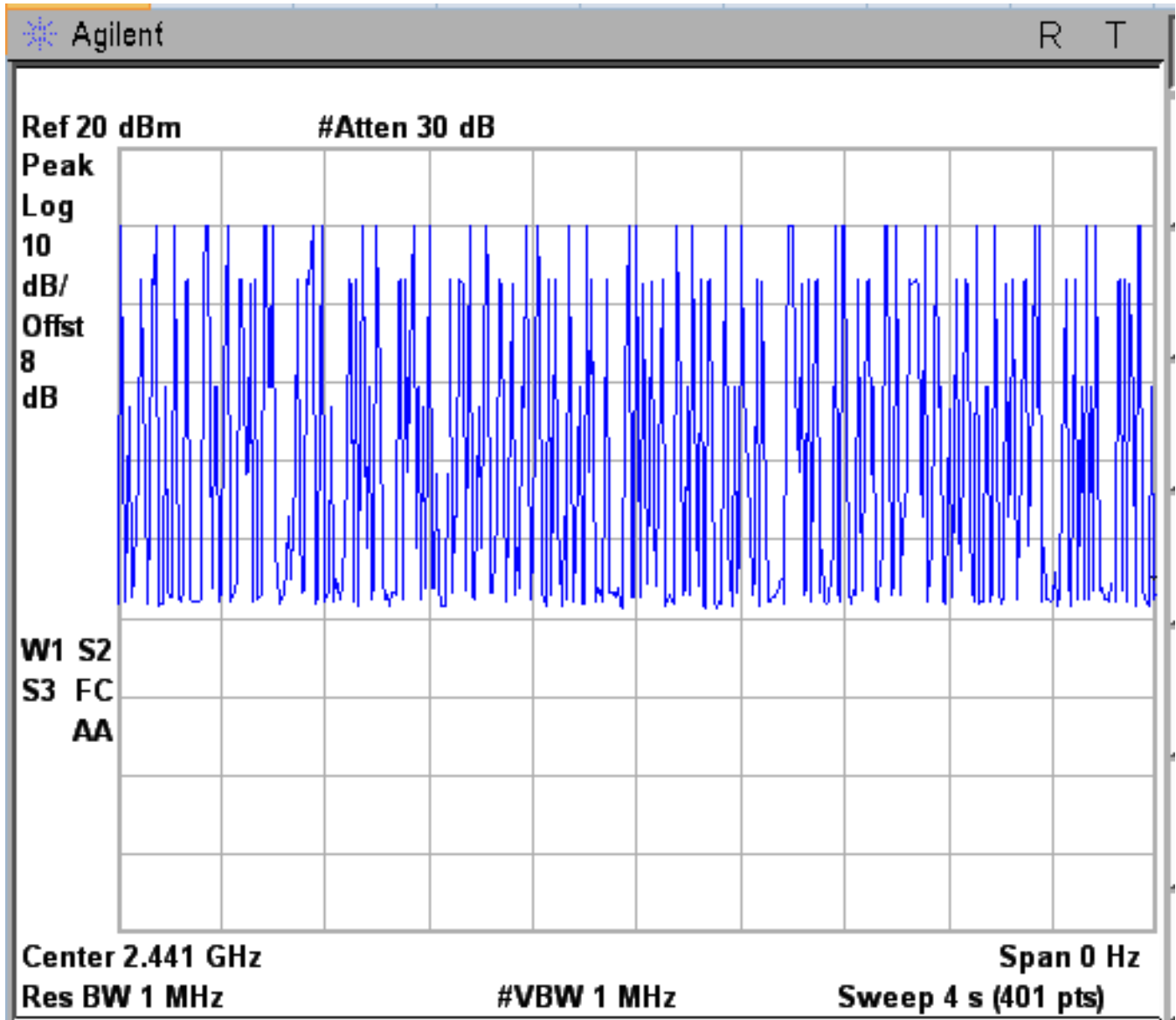
Figure 6d.4-2: Plot of dwell time over 4 second period.
