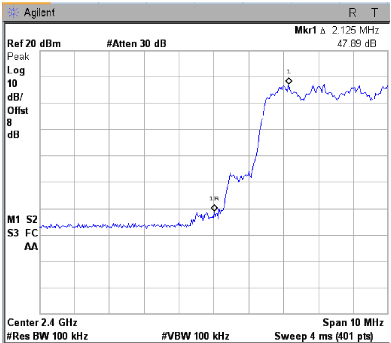
Figure 6d.6-7: Plot of lower band-edge conducted emissions with hopping enabled (Pi/4 DPSK Modulation).
