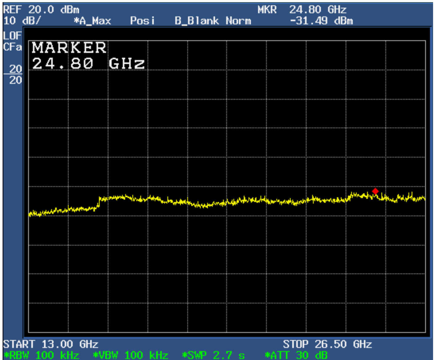
Figure 6d.7-3: Plot of spurious conducted emissions 13 GHz – 26.5 GHz (Low channel enabled).
