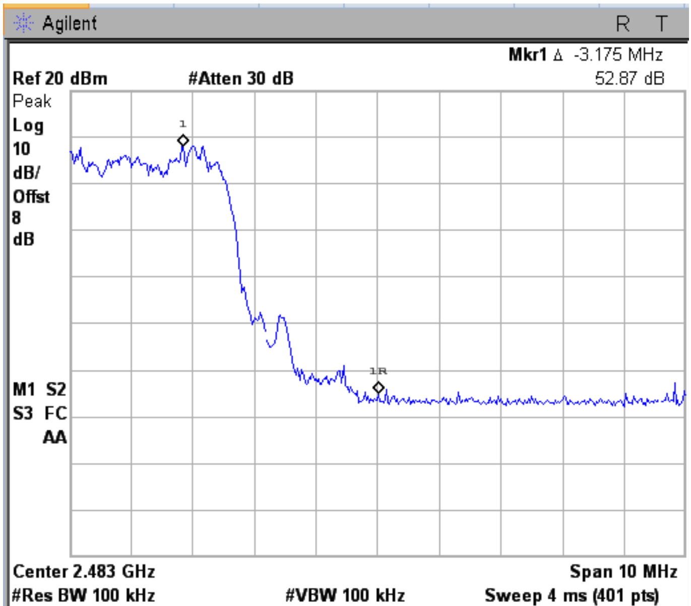
Figure 6d.6-12: Plot of upper band-edge conducted emissions with hopping enabled (8 DPSK Modulation).
