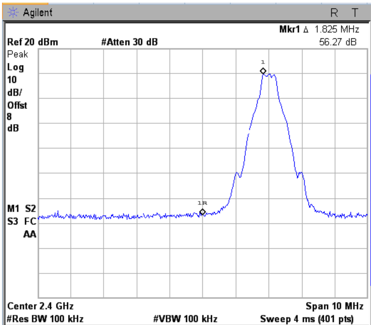
Figure 6d.6-1: Plot of lower band-edge conducted emissions with hopping disabled (GFSK Modulation).
