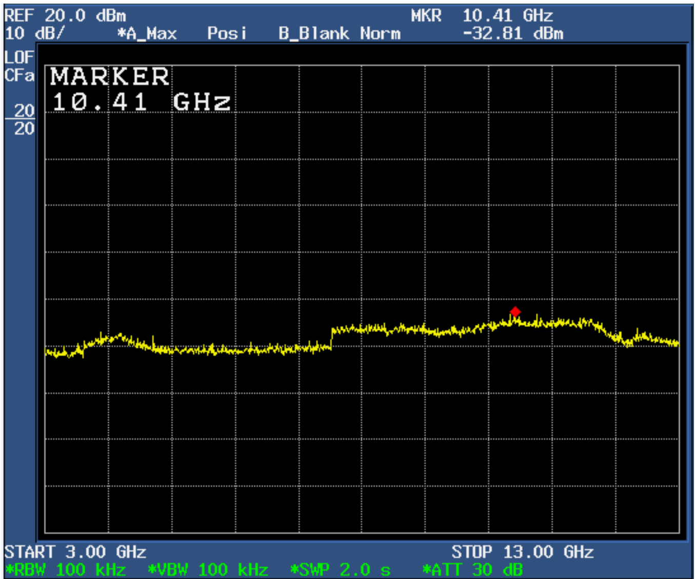
Figure 6d.7-5: Plot of spurious conducted emissions 3 GHz – 13 GHz (Mid channel enabled).
