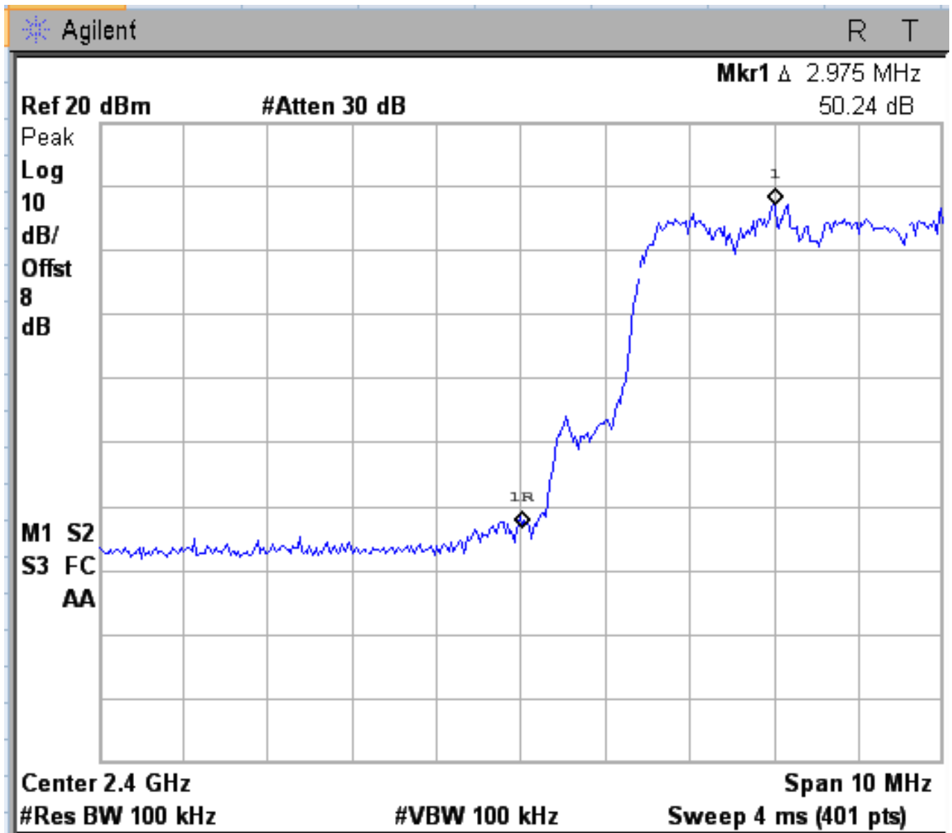
Figure 6d.6-11: Plot of lower band-edge conducted emissions with hopping enabled (8 DPSK Modulation).
