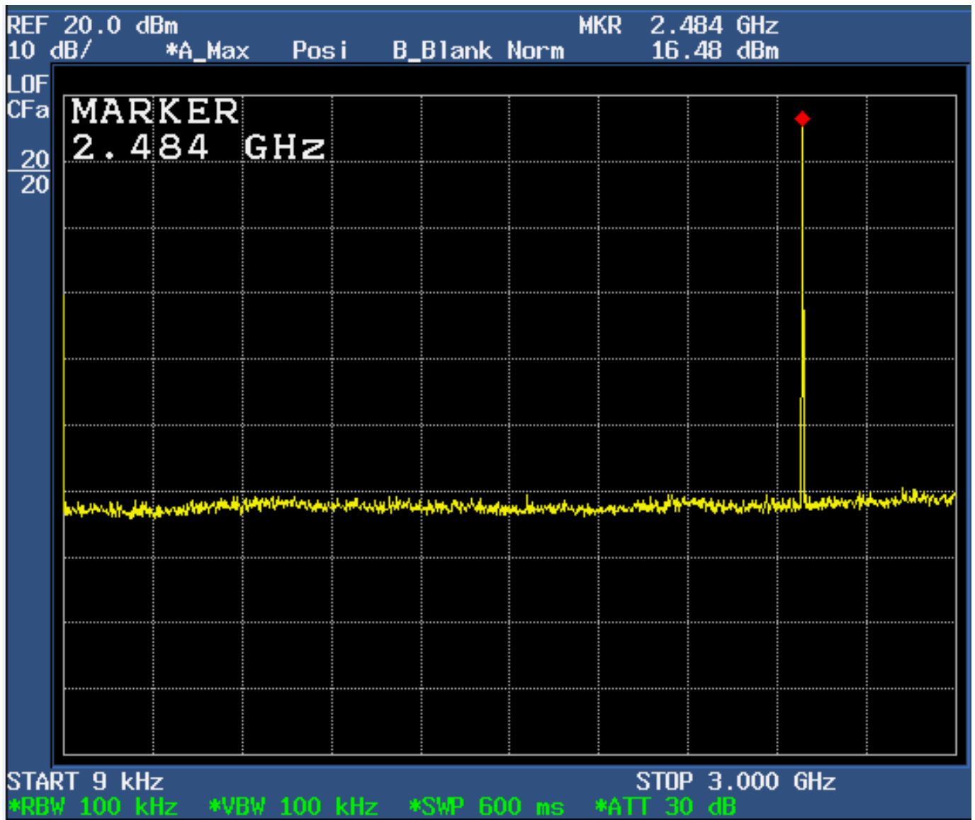
Figure 6d.7-7: Plot of spurious conducted emissions 9.0 kHz – 3.0 GHz (High channel enabled).
