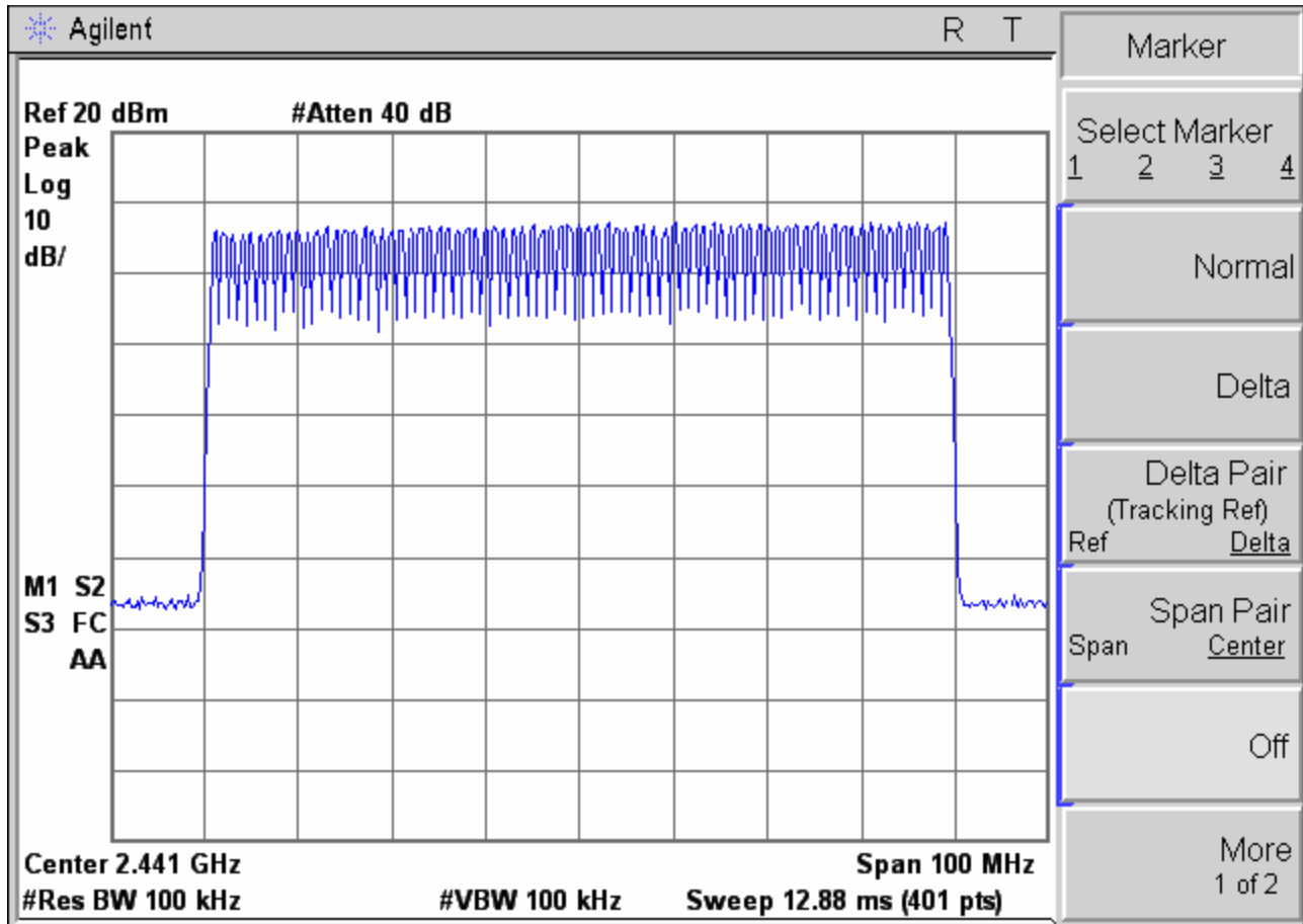
Figure 6d.3-1: Plot of number of Bluetooth hopping frequencies
