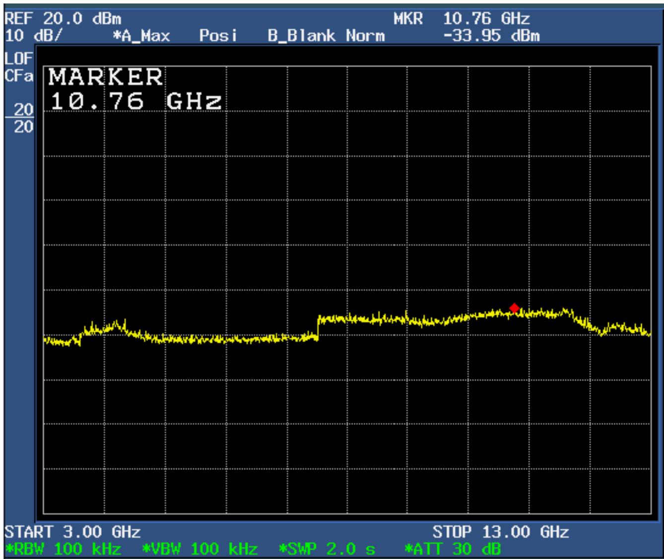
Figure 6d.7-2: Plot of spurious conducted emissions 3 GHz – 13 GHz (Low channel enabled).
