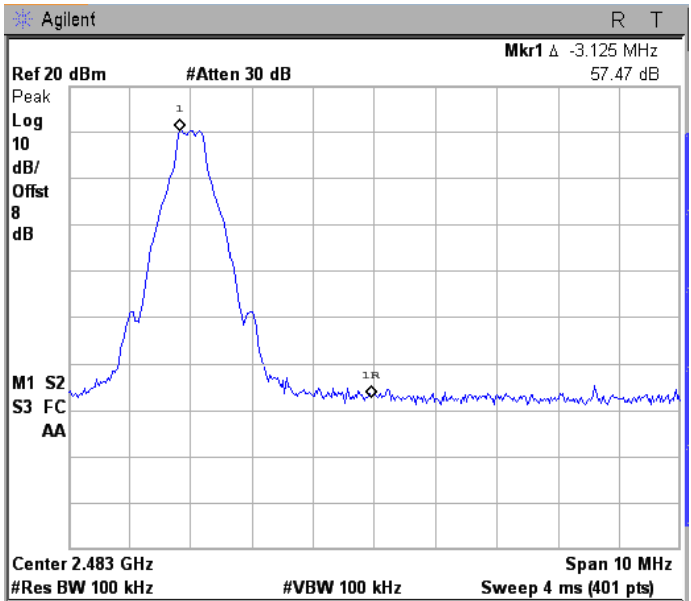
Figure 6d.6-2: Plot of upper band-edge conducted emissions with hopping disabled (GFSK Modulation).
