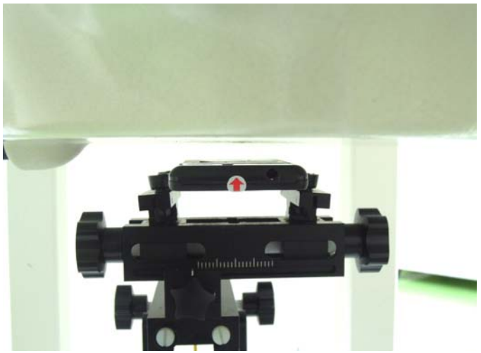
Rear Face of DUT with 1.0 cm Gap (Hotspot)
