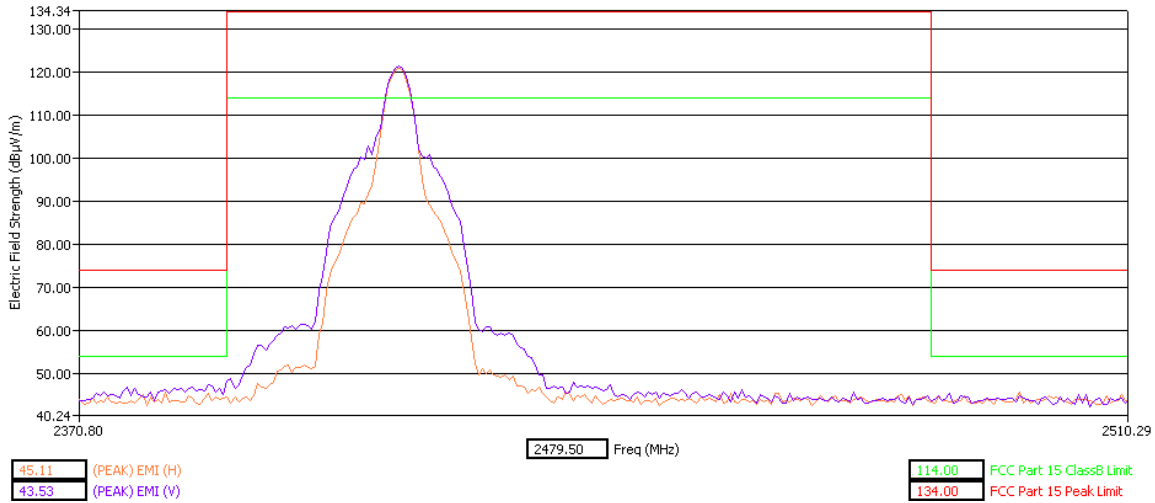
Low Band Edge X Orientation Peak Detector
