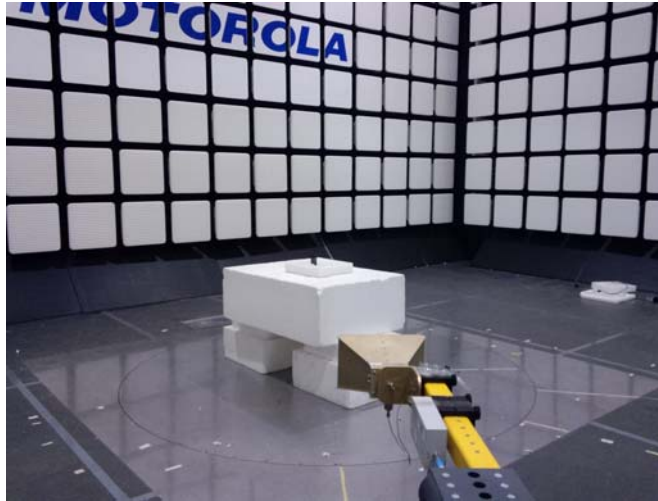
Radiated Emissions
