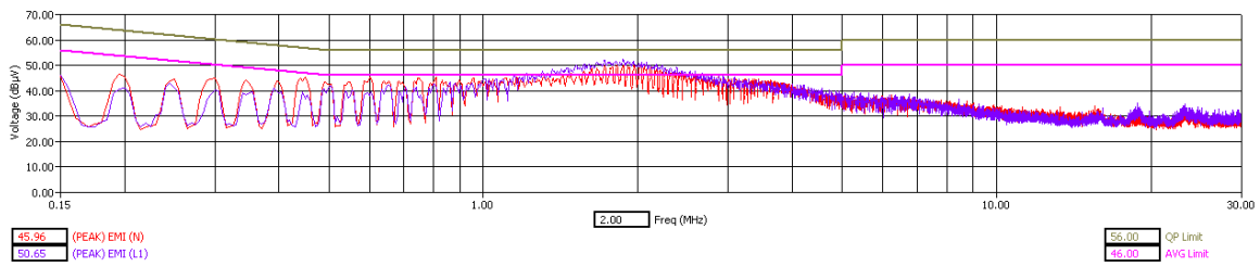
Bluetooth – Hopping - Tx Mode – Peak Detector
