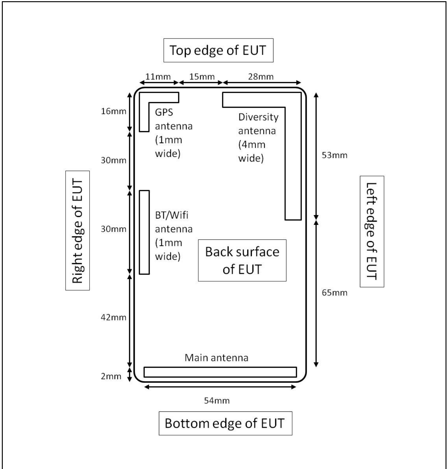
Figure 9-6: Antenna Locations and Spacings.
