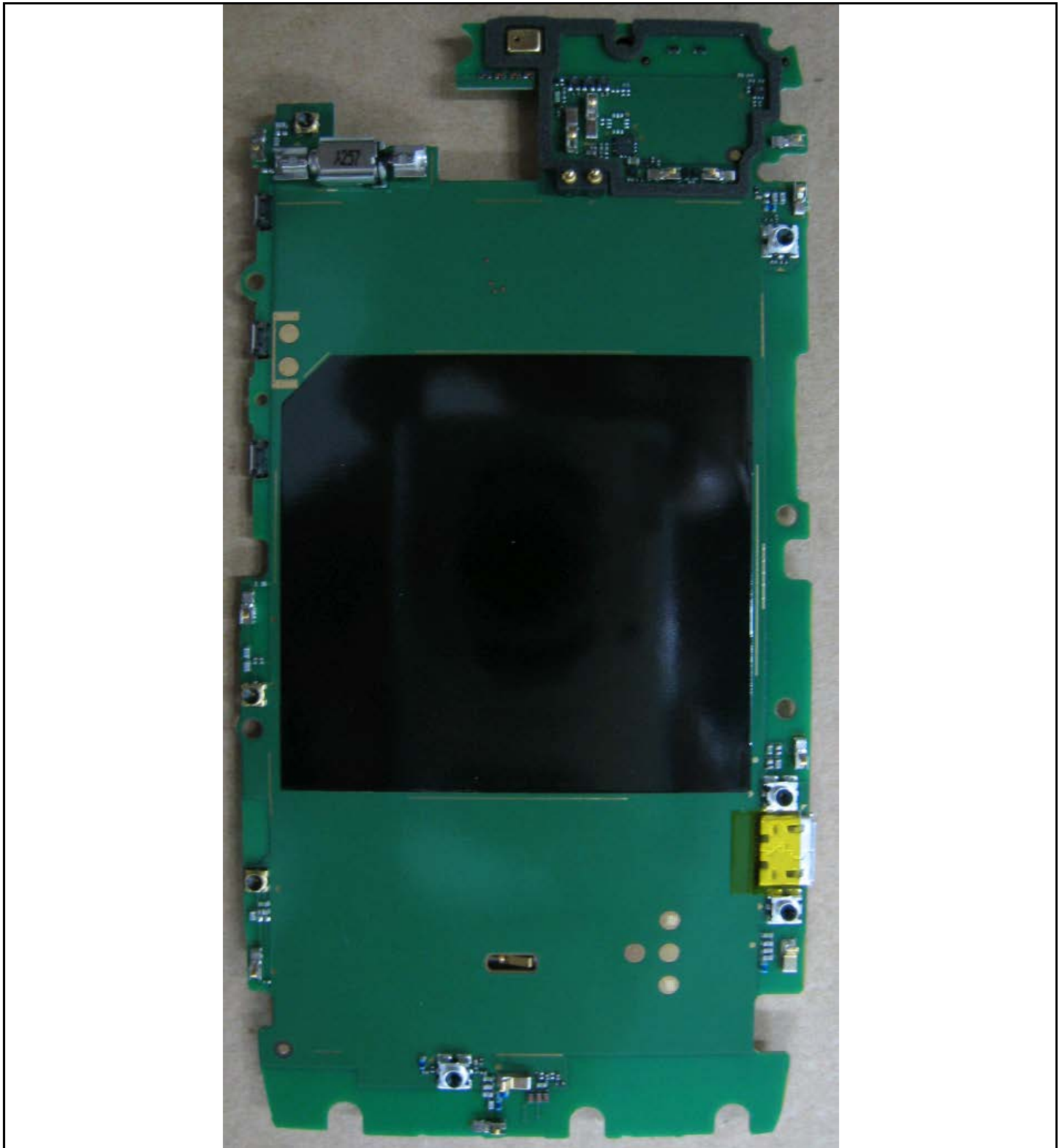
Photograph 9-3: Front side view of the device's PC Board.
