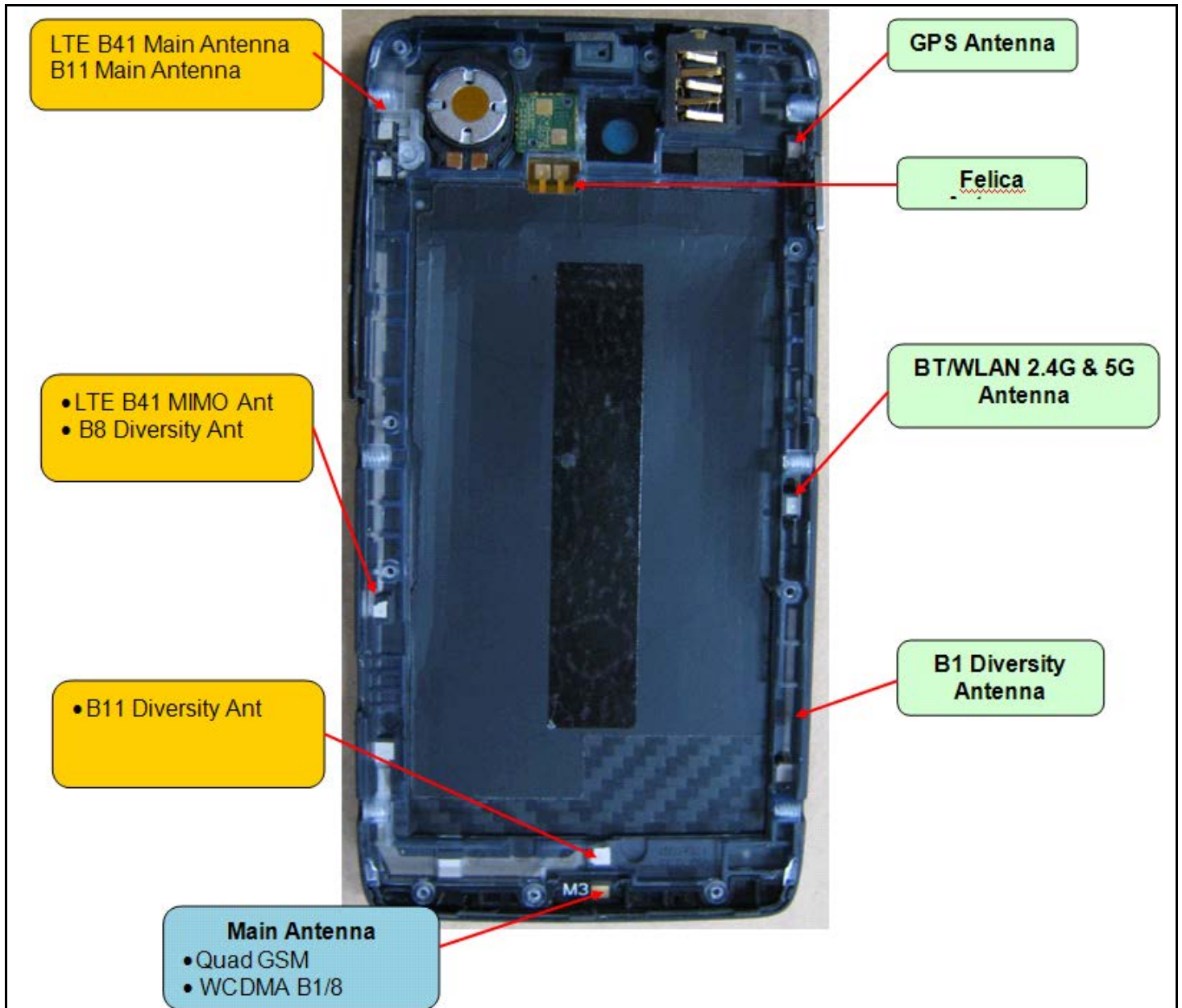
Photograph 9-4: Interior Housing View, Showing Antenna Locations.
