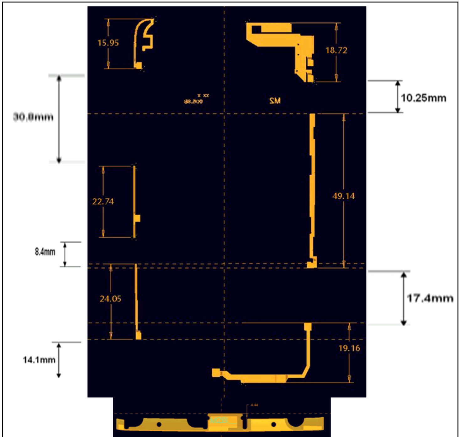
Photograph 9-6: Antenna Locations and Spacings.
