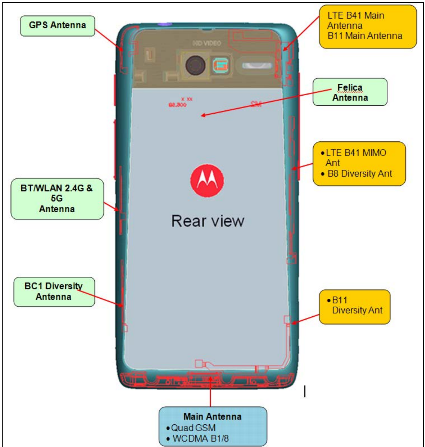
Photograph 9-5: Antenna Locations Schematic.
