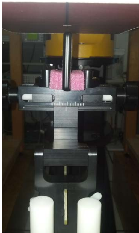
Figure 9: Mobile Hotspot Position, Long Edge of Phone facing Phantom (10 mm separation)
