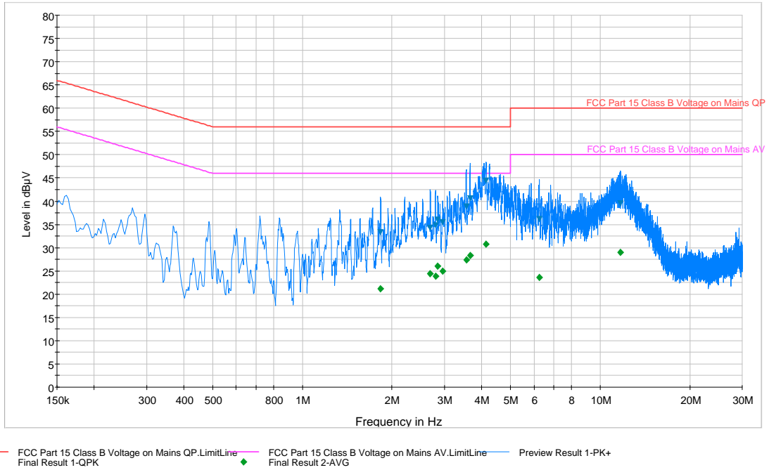
Plot 6-63. Line Conducted Plot with 802.11a (L1)
