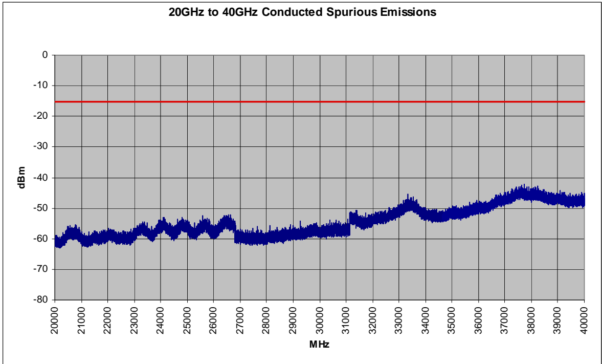
Plot 6-56. Conducted Spurious Plot (802.11a – Ch. 149)
