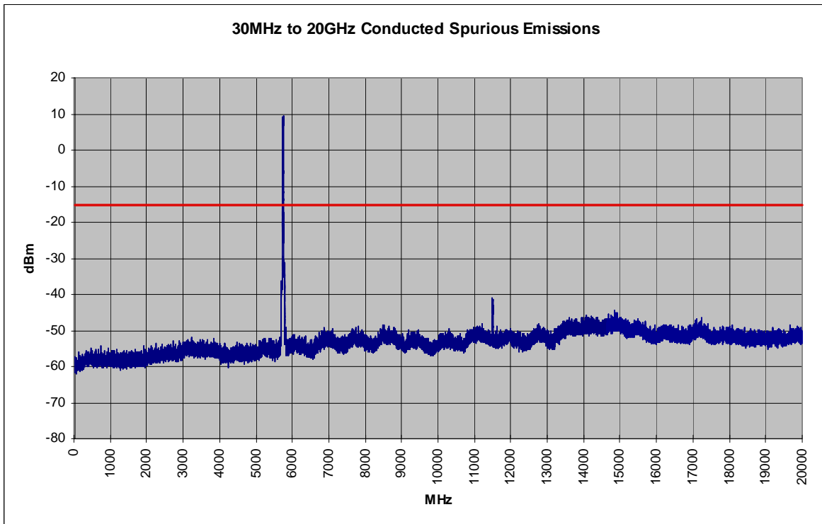
Plot 6-55. Conducted Spurious Plot (802.11a – Ch. 149)
