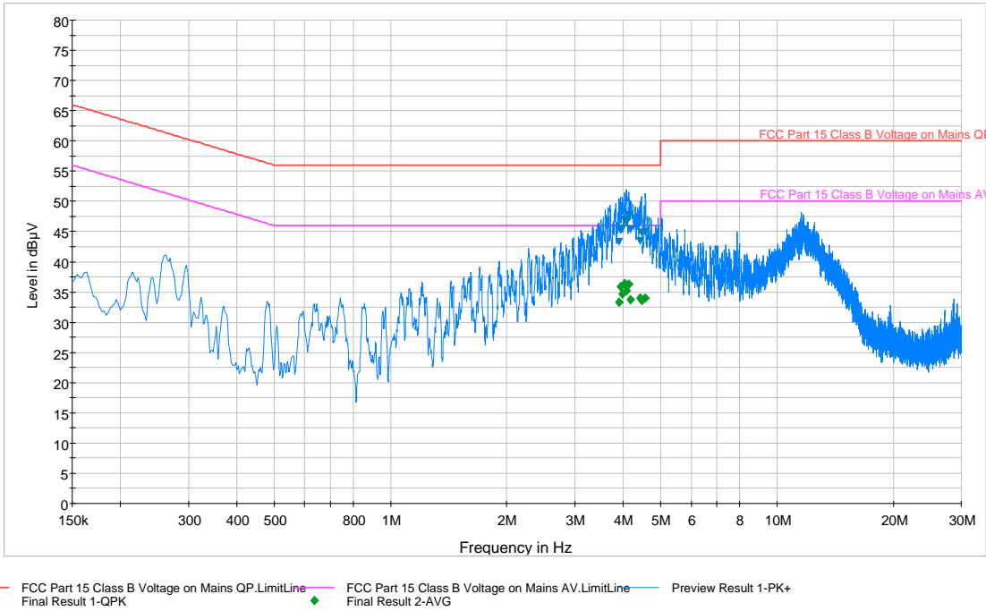
Plot 6-64. Line Conducted Plot with 802.11a (N)
