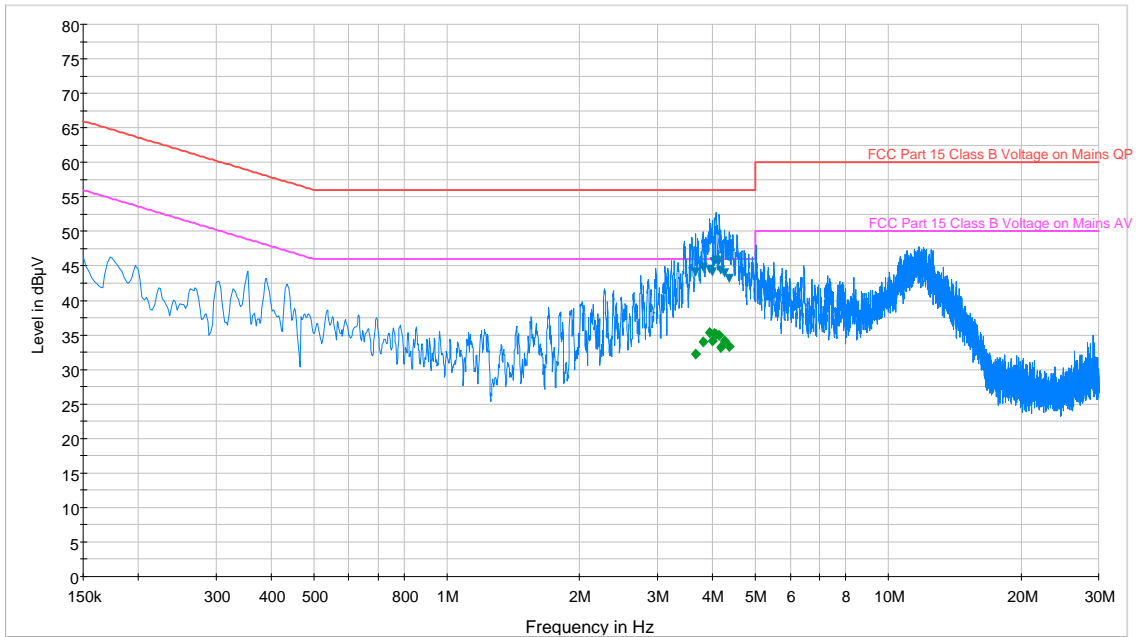
Plot 6-62. Line Conducted Plot with 802.11b (N)
