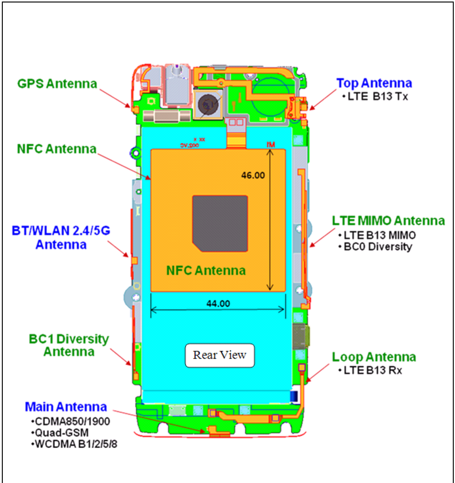
Photograph 9-6: Antenna Locations, Schematically.
