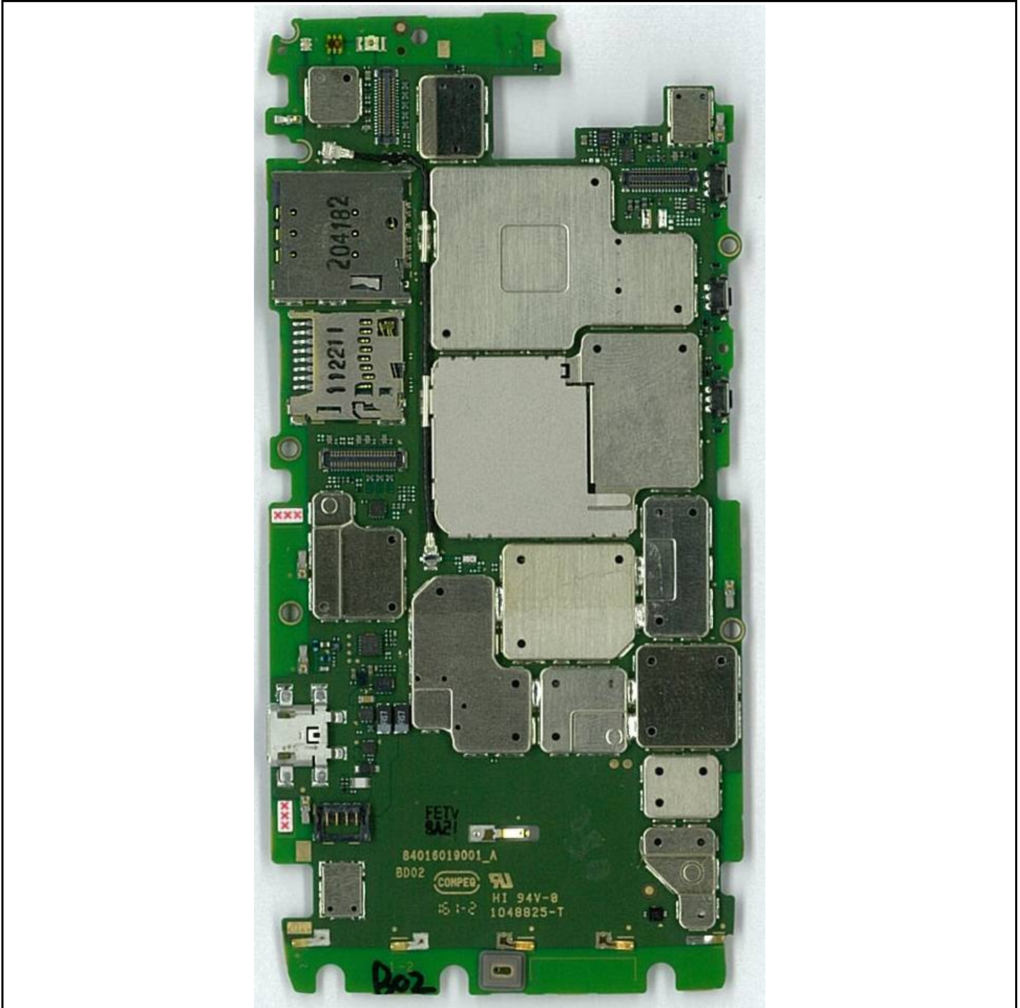
Photograph 9-1: Front side view of the device's PC Board, Shields in place.
