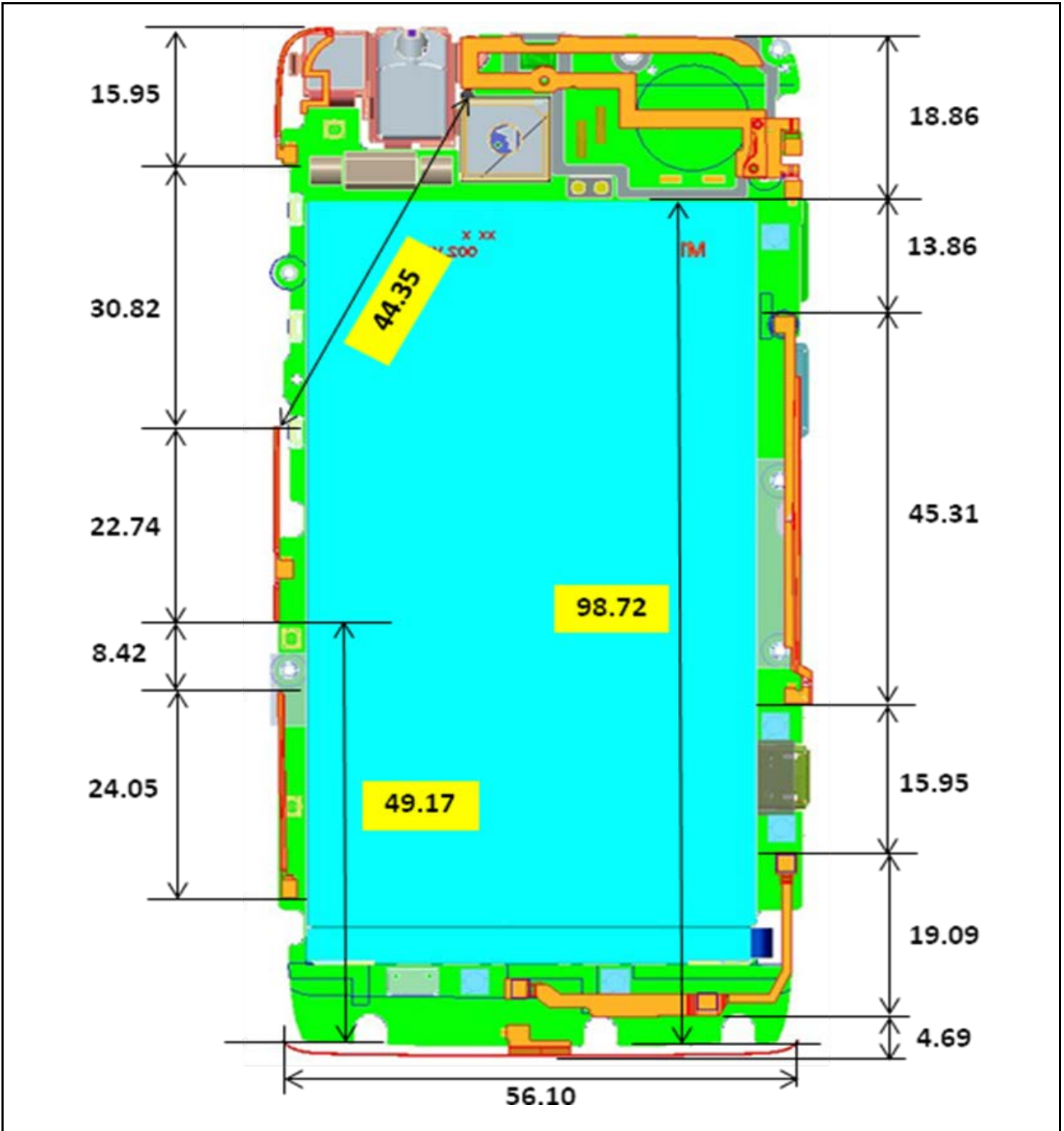
Photograph 9-7: Distances between Key Antennas.
