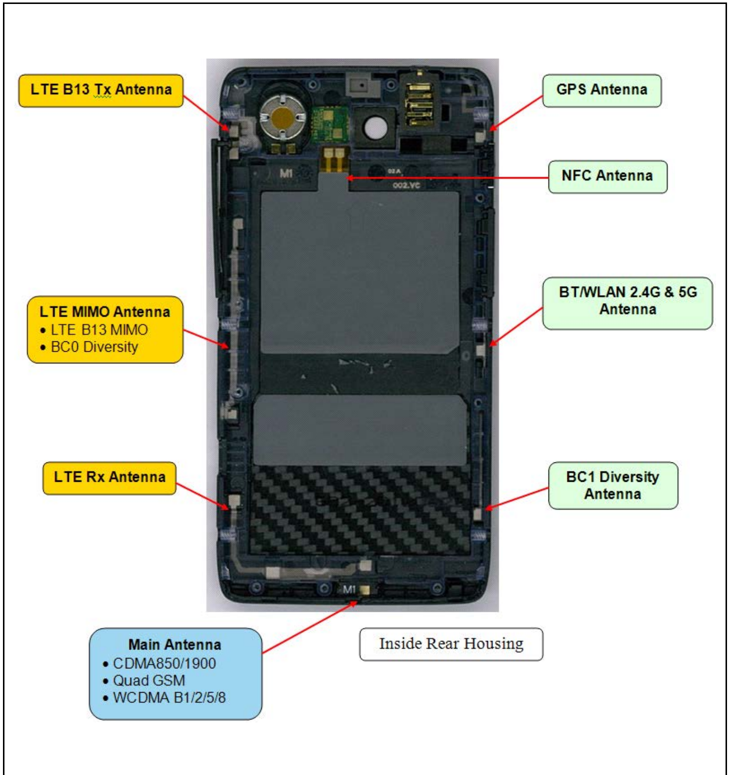
Photograph 9-5: Antenna Locations.
