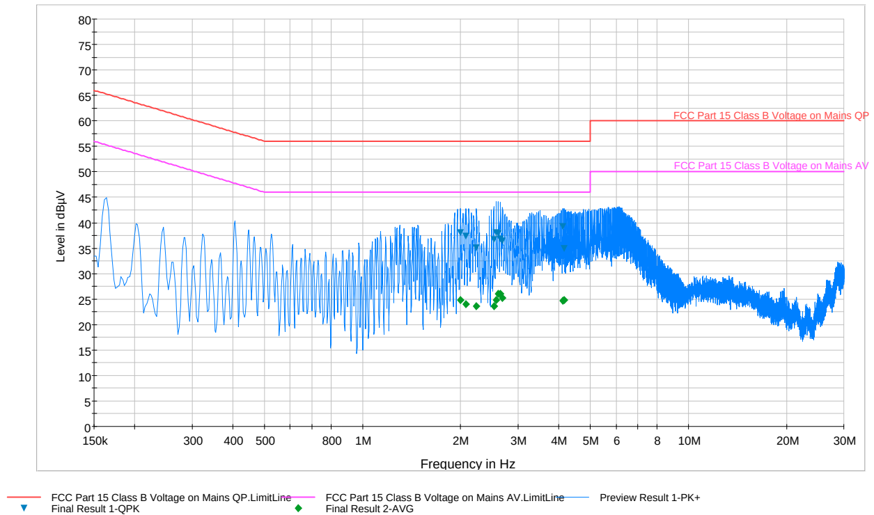
Plot 6-25. Line-Conducted Test Plot (N)
