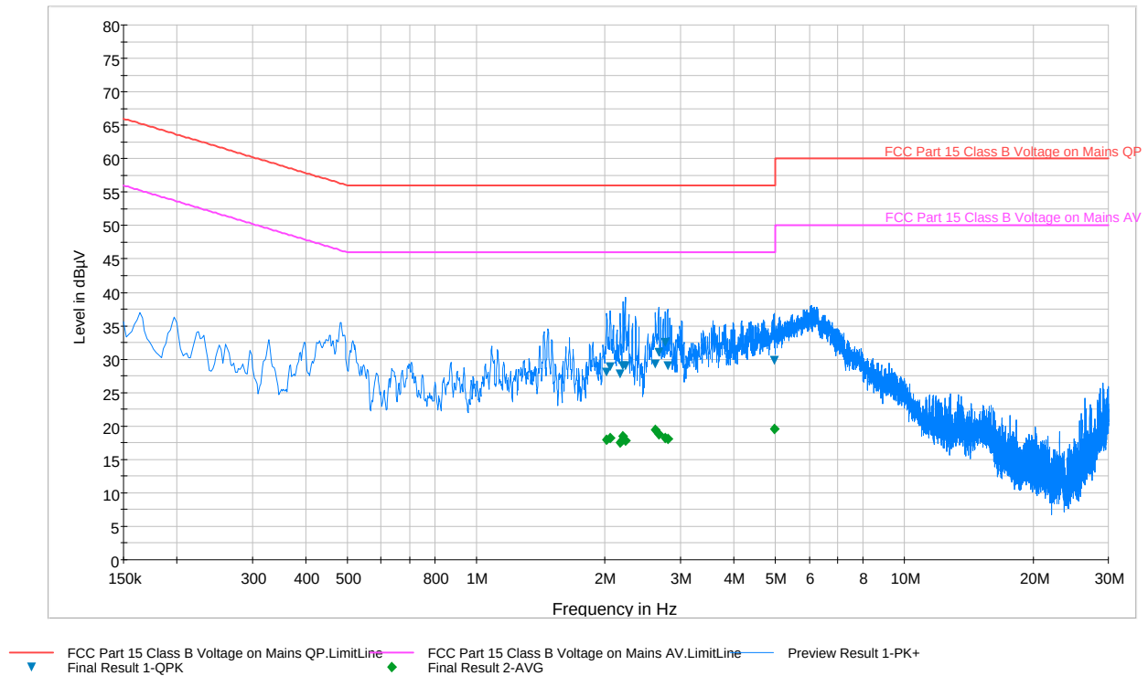
Plot 6-24. Line-Conducted Test Plot (L1)
