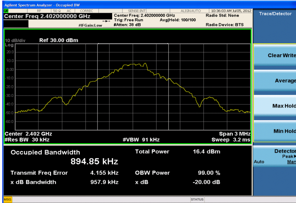
Plot 6-1. 20dB Bandwidth Plot (Bluetooth, 1Mbps – Ch. 0)
