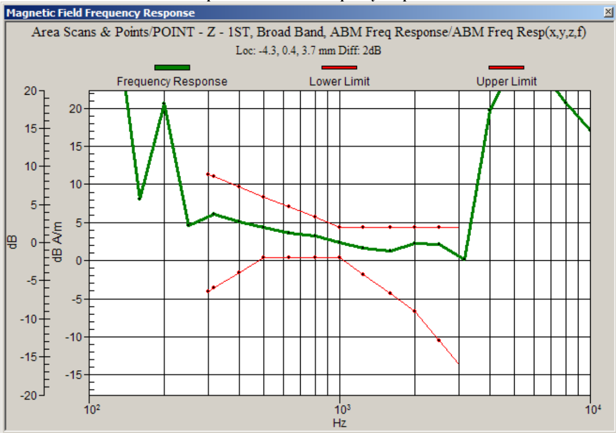
Graph 3: CDMA 1900 Frequency Response
