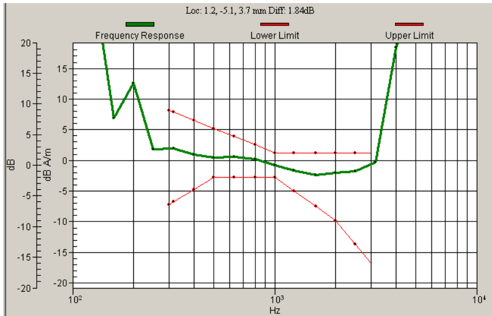
Graph 3: WCDMA 1700 Frequency Response
