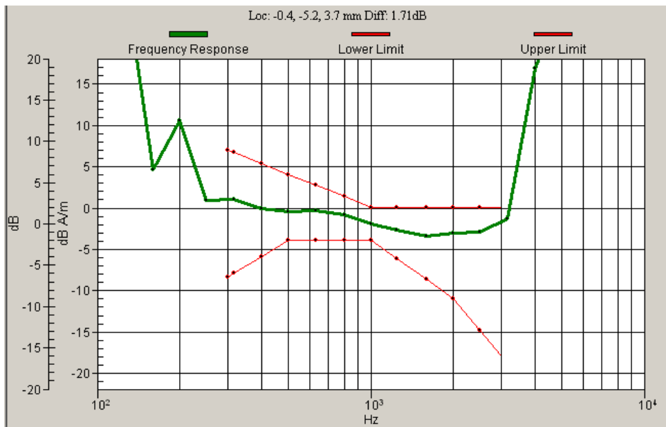
Graph 3: WCDMA 1900 Frequency Response
