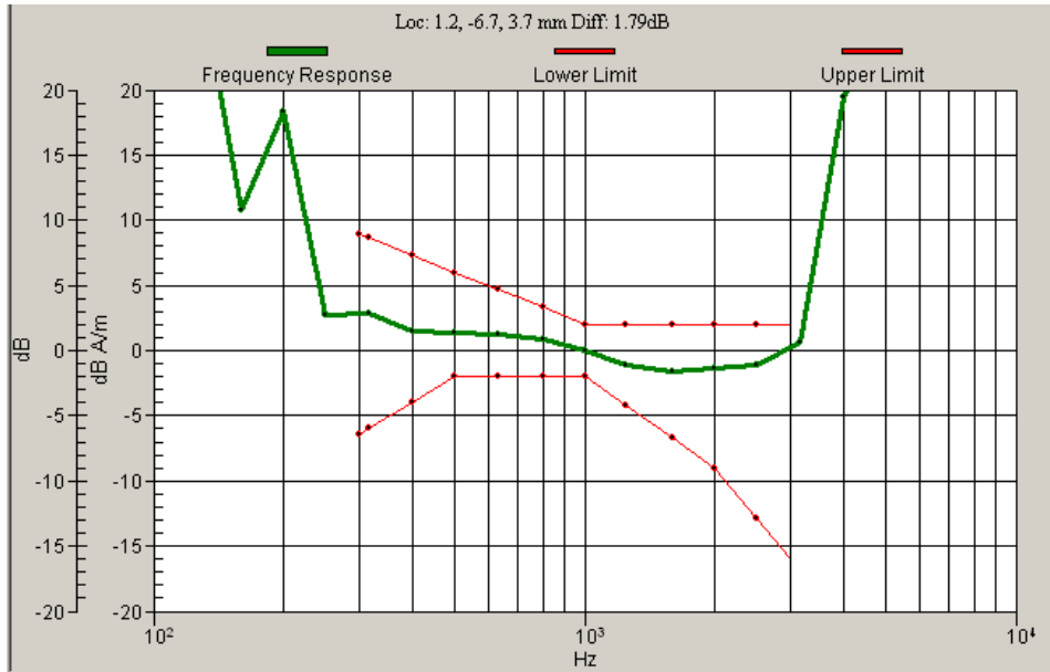
Graph 2: GSM 1900 Frequency Response
