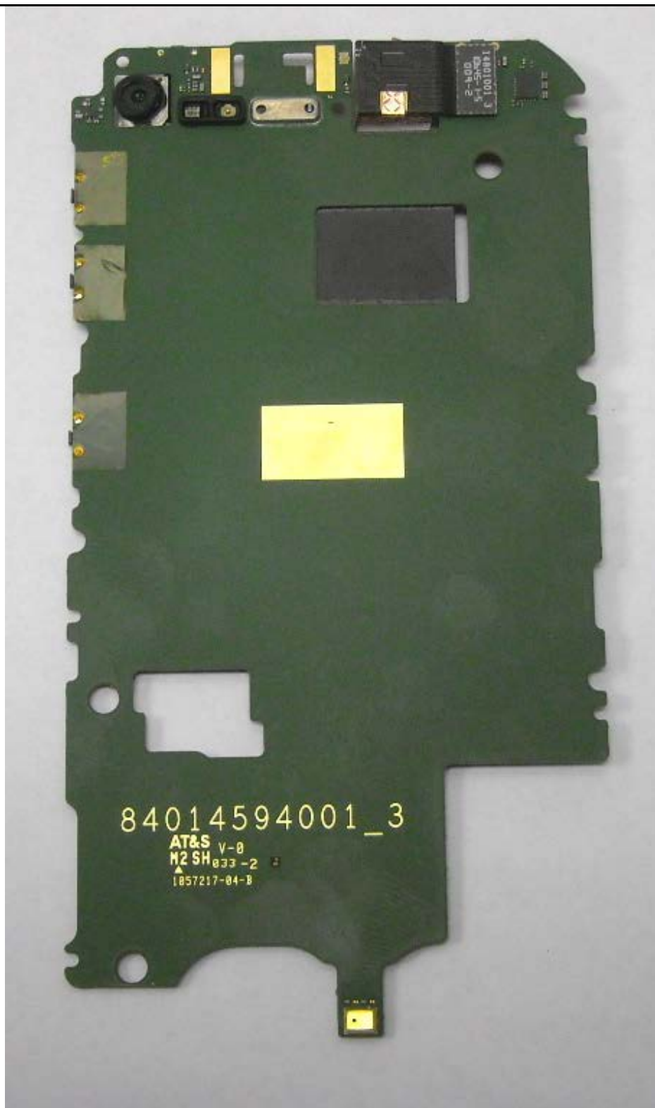
Photograph 9-5: Front side view of the device's auxiliary PC Board.
