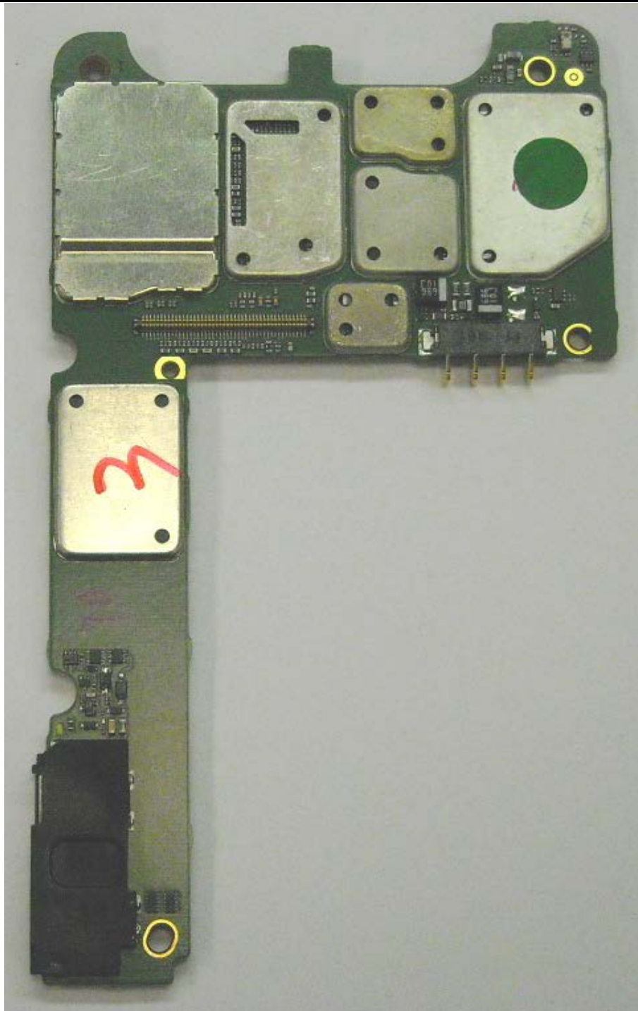
Photograph 9-1: Front side view of the device's main PC Board, Shields in place.
