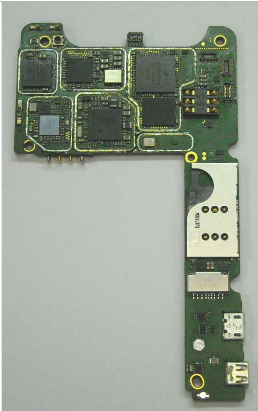
Photograph 9-4: Back side view of the device's main PC Board, Shields Removed.
