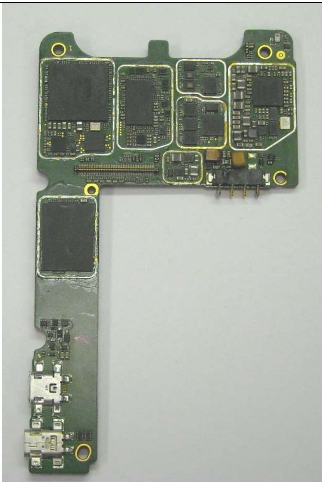
Photograph 9-3: Front side view of the device's main PC Board, Shields Removed.
