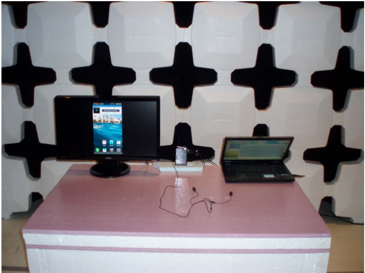
Radiated - JBP
