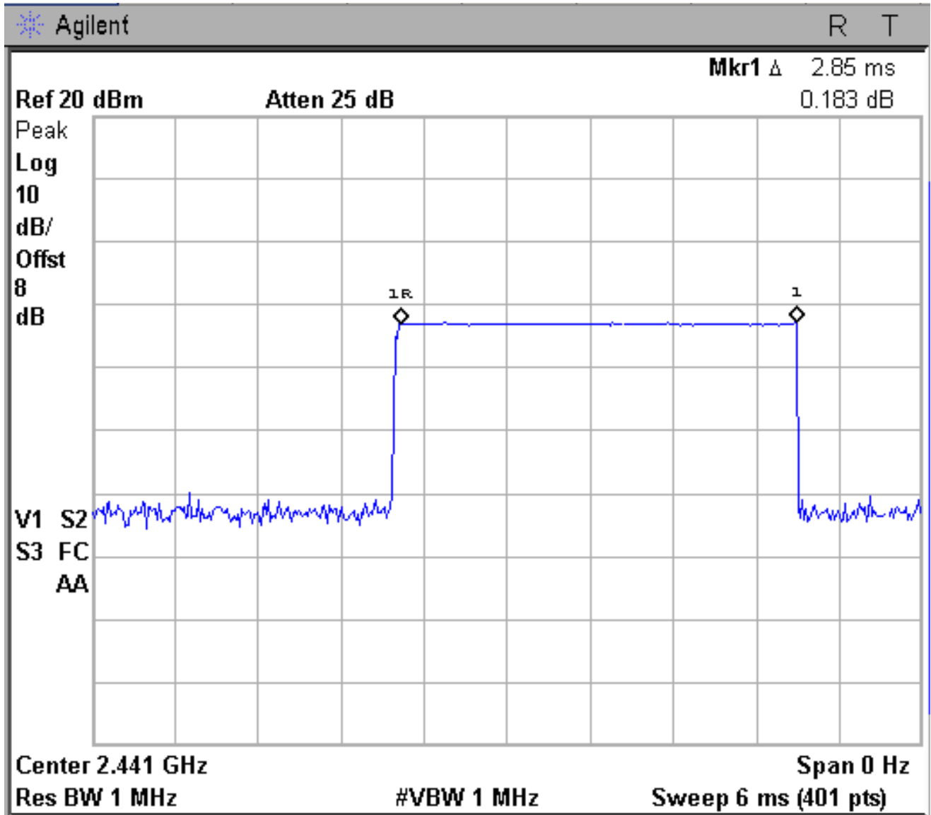
Figure 6c.4-4: Plot of dwell time over 6ms period.
