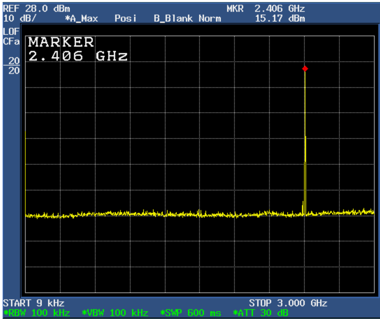
Figure 6d.7-1: Plot of spurious conducted emissions Plot of spurious conducted emissions 9 kHz – 3.0 GHz (Low Channel Enabled).
