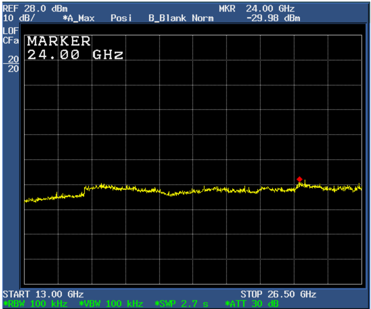
Figure 6d.7-6: Plot of spurious conducted emissions 13 GHz – 26.5 GHz (Mid Channel Enabled).
