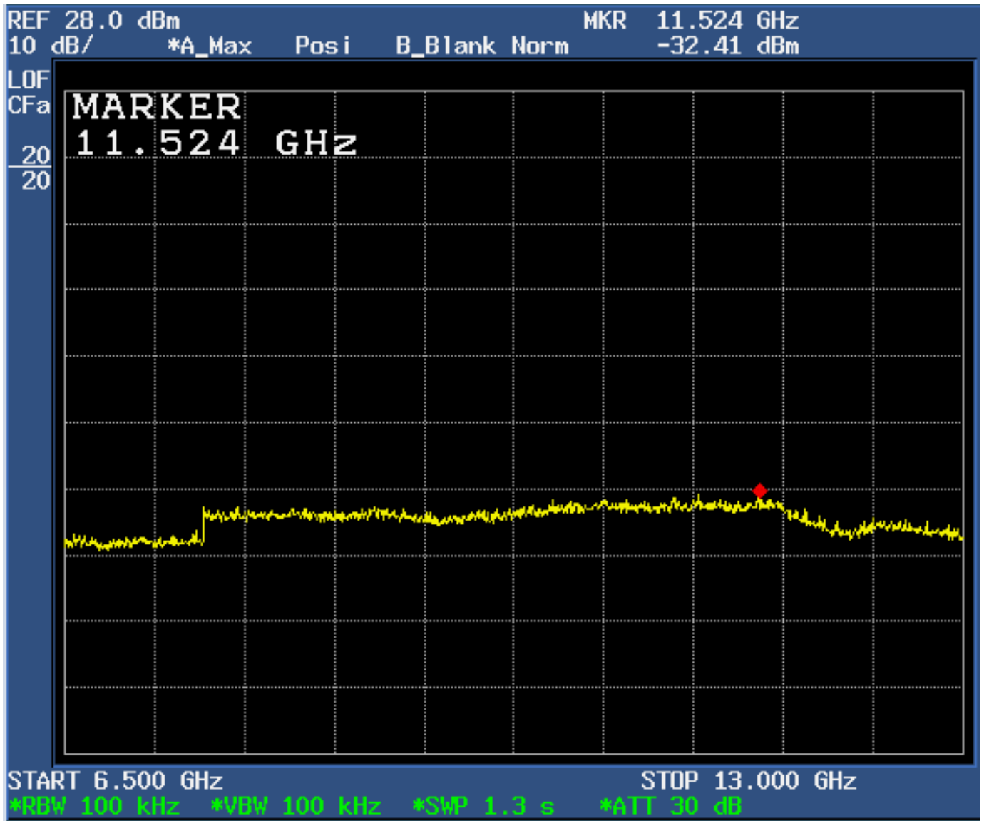
Figure 6d.7-12: Plot of spurious conducted emissions 6.5 GHz – 13.0 GHz (Hopping Enabled).
