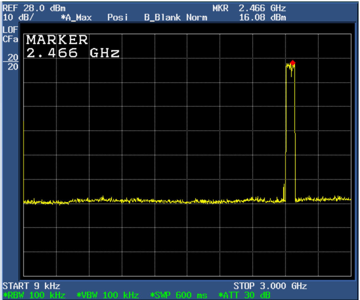
Figure 6d.7-10: Plot of spurious conducted emissions 9 kHz – 3.0 GHz (Hopping Enabled).
