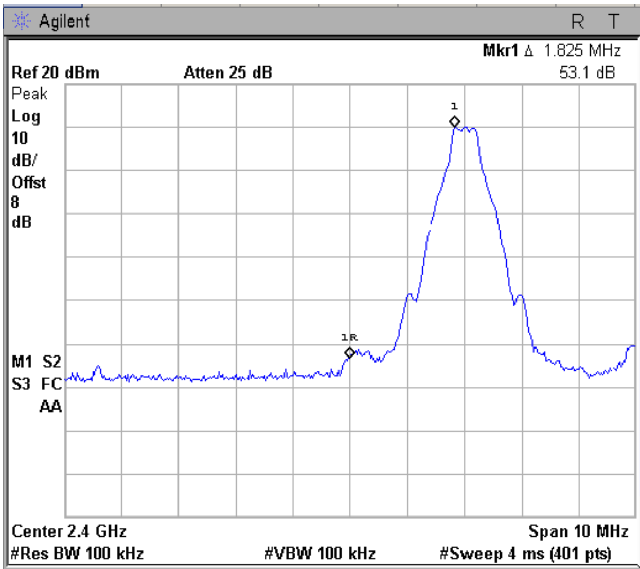
Figure 6d.6-1: Plot of lower band-edge conducted emissions with hopping disabled (GFSK Modulation).
