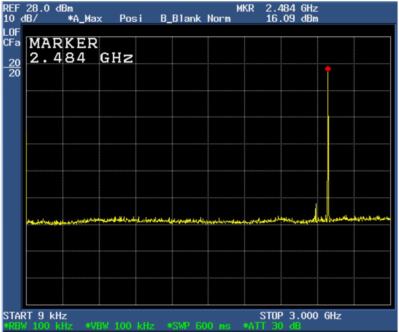
Figure 6d.7-7: Plot of spurious conducted emissions 9 kHz – 3.0 GHz (High Channel Enabled).
