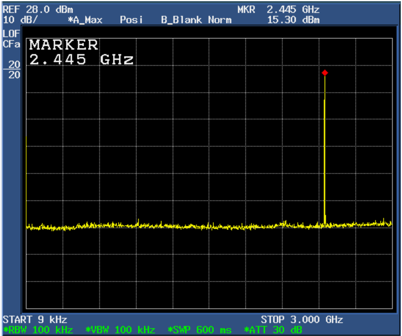
Figure 6d.7-4: Plot of spurious conducted emissions Plot of spurious conducted emissions 9 kHz – 3.0 GHz (Mid Channel Enabled).
