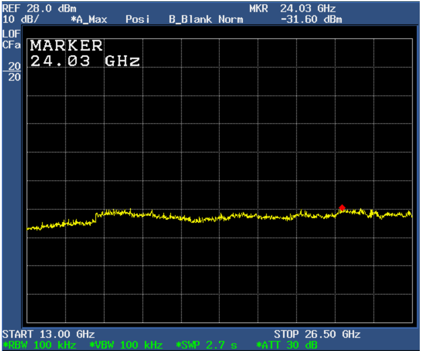
Figure 6d.7-13: Plot of spurious conducted emissions 13 GHz – 26.5 GHz (Hopping Enabled).
