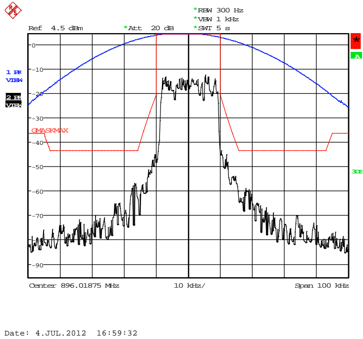
Figure 6a-2.2.1. iDEN 900 MHz Band, QPSK, Maximum Power, Emission Mask G
