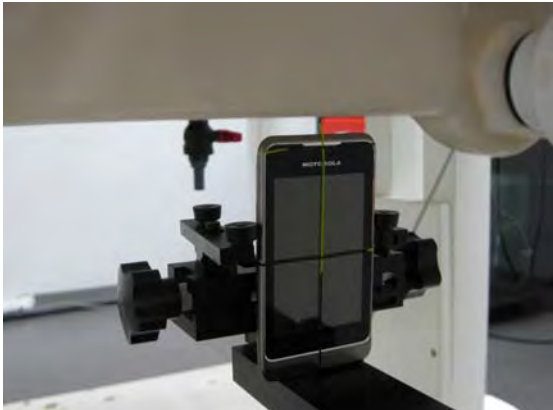
Fig.10 EUT Top to flat phantom
