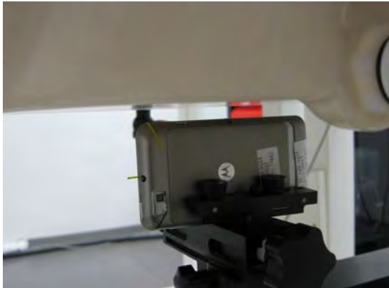
Fig.13 EUT Left to flat phantom
