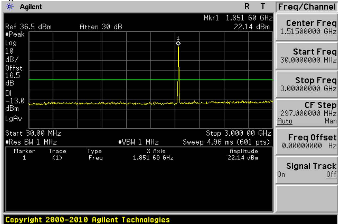
Figure 9-26: Out of Band emission at antenna terminals–HSDPA II Channel Lowest
