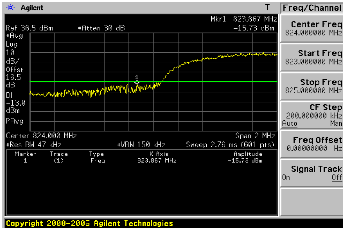
Figure 9-49: Bad edge emission at antenna terminals –HSUPA V Channel Lowest
