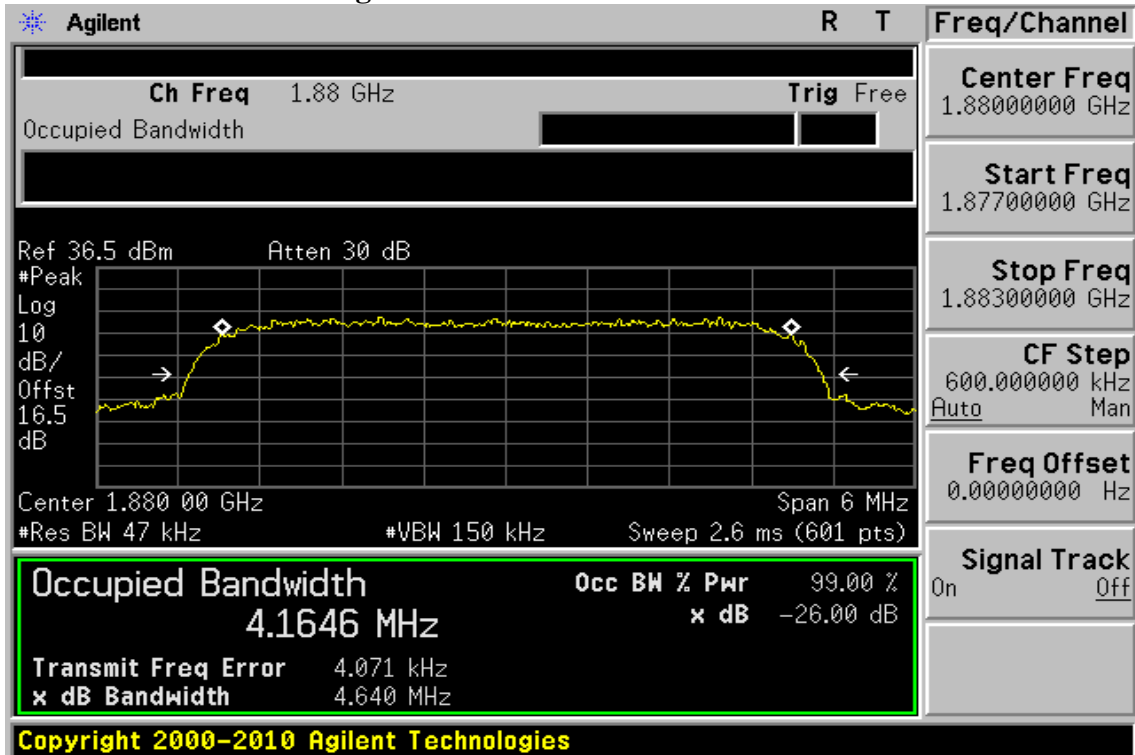
Figure 8-17 HSDPA II Channel Mid
