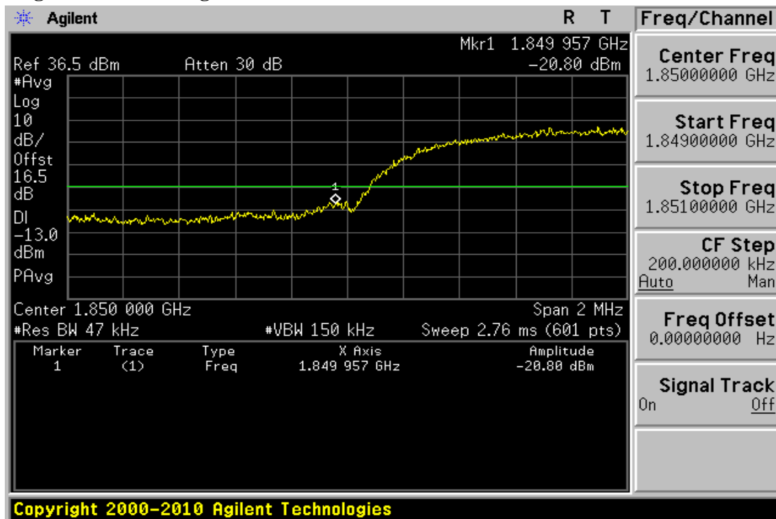
Figure 9-29: Bad edge emission at antenna terminals –HSDPA II Channel Lowest
