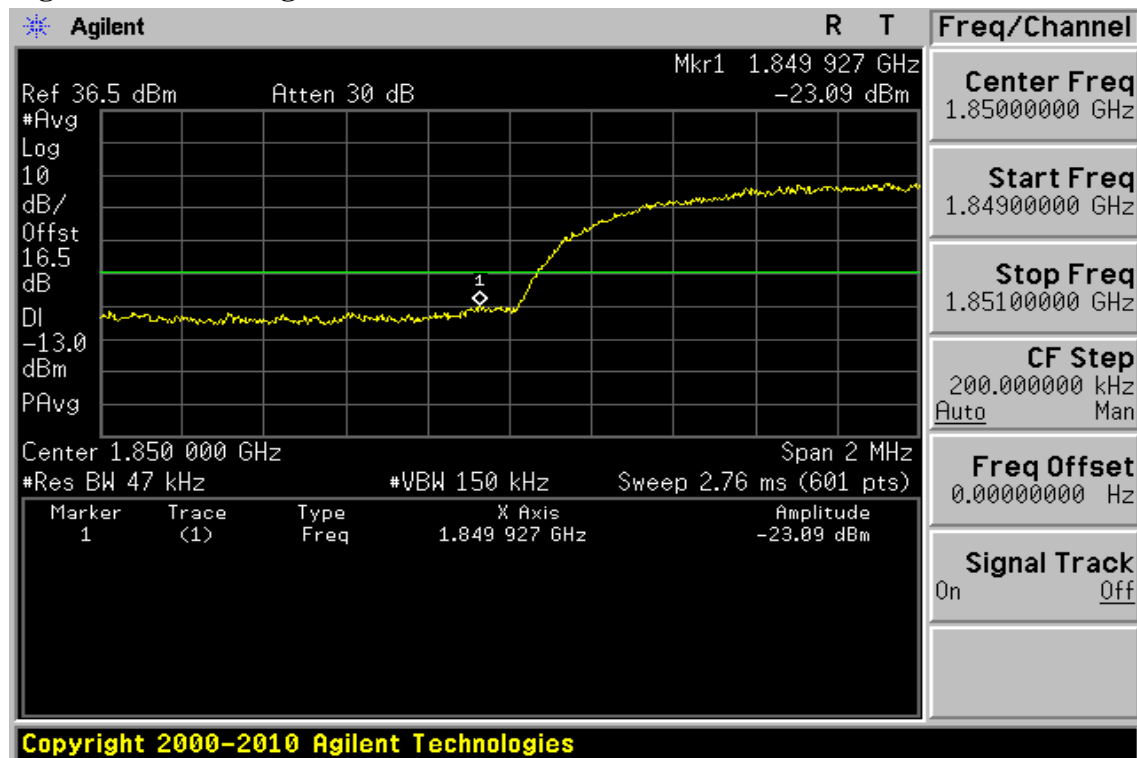
Figure 9-24: Bad edge emission at antenna terminals –WCDMA II Channel Lowest
