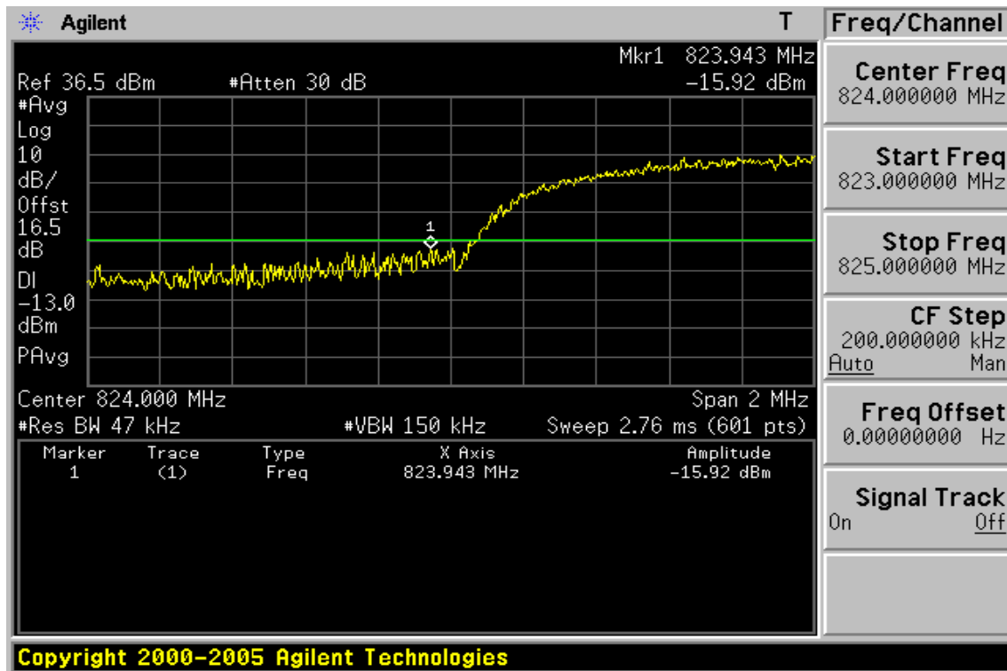
Figure 9-44: Bad edge emission at antenna terminals –HSDPA V Channel Lowest
