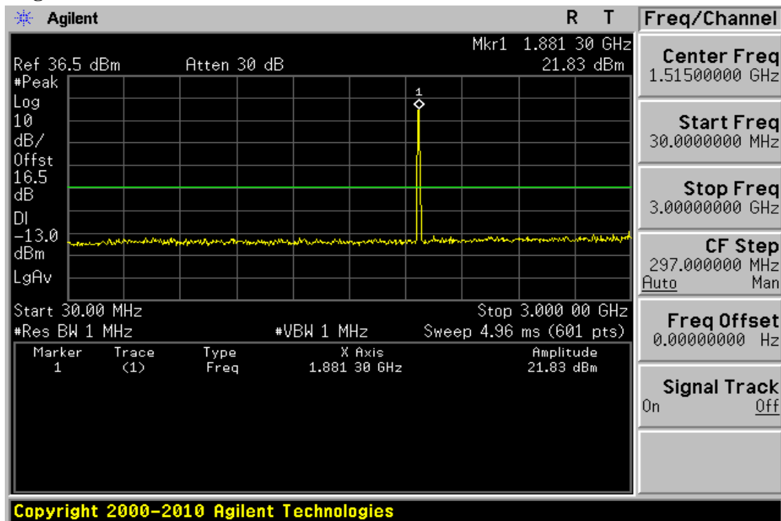
Figure 9-27: Out of Band emission at antenna terminals –HSDPA II Channel Mid
