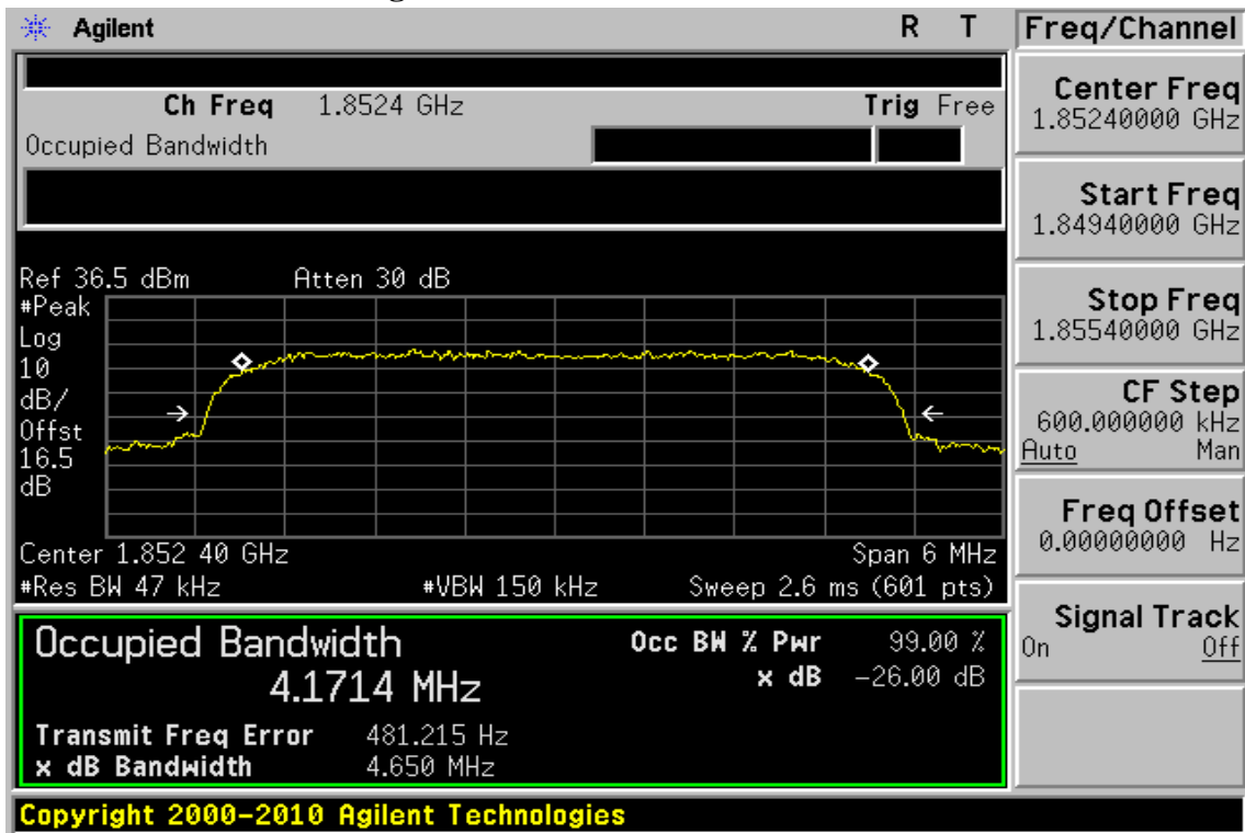
Figure 8-19 HSUPA II Channel Low
