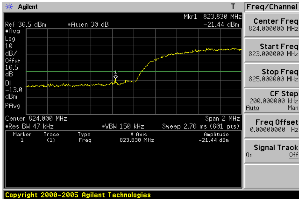
Figure 9-39: Bad edge emission at antenna terminals –WCDMA V Channel Lowest
