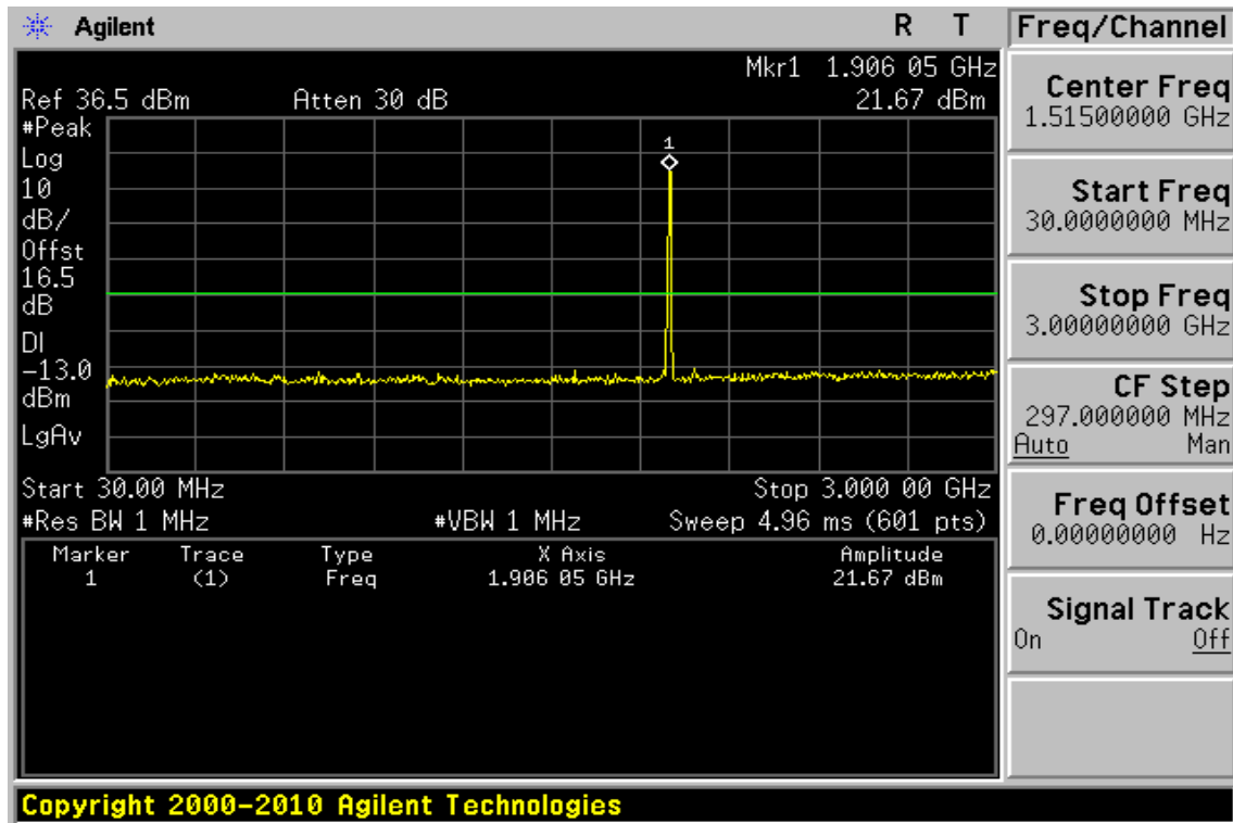
Figure 9-28: Out of Band emission at antenna terminals–HSDPA II Channel Highest
