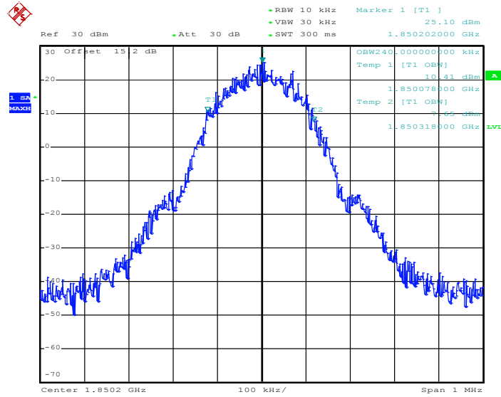
99% Occupied Bandwidth Plot on Channel 512
