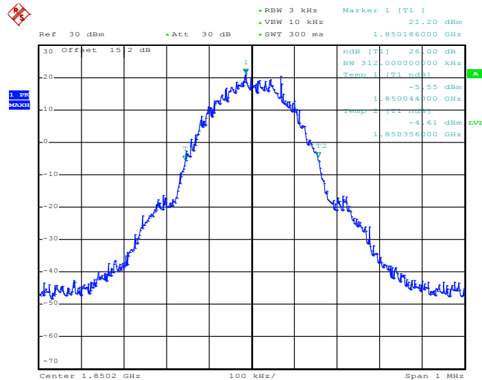
26dB Bandwidth Plot on Channel 512
