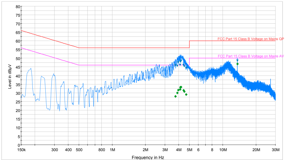
Plot 8-1. Line-Conducted Test Plot (L1)
