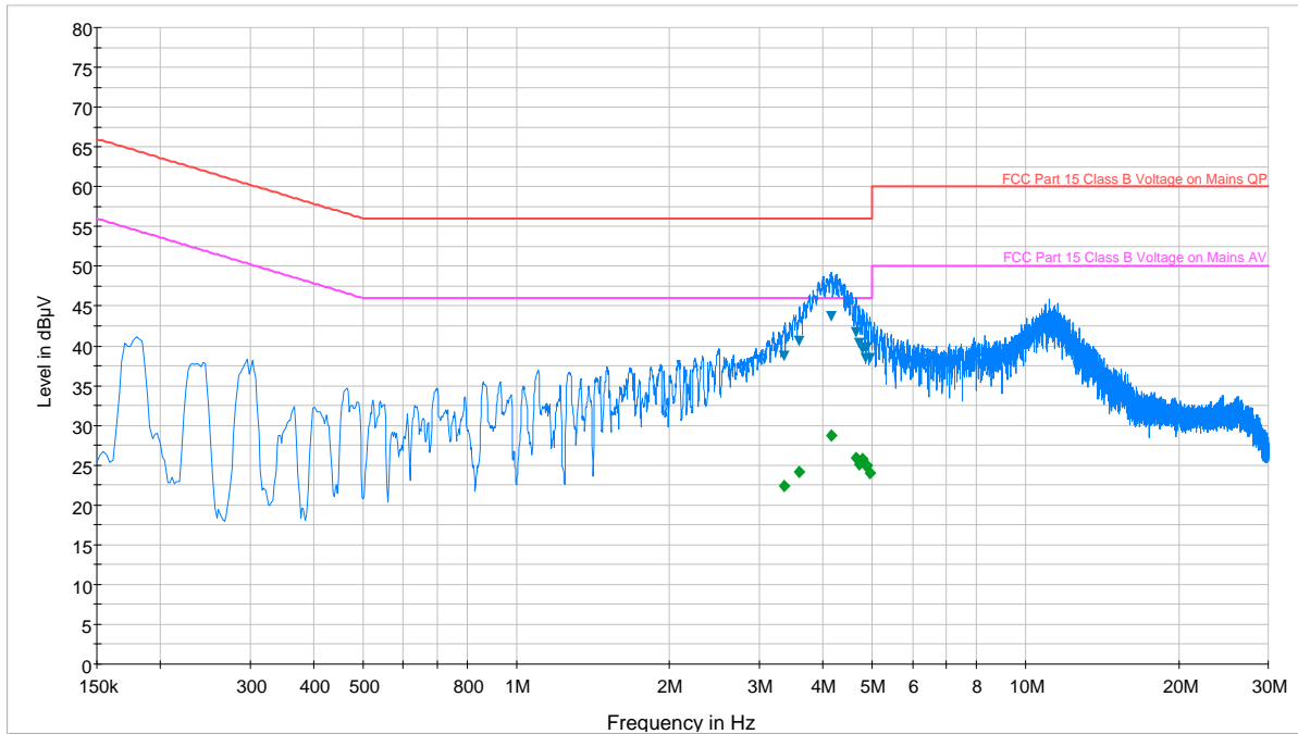
Plot 6-24. Line-Conducted Test Plot (L1)
