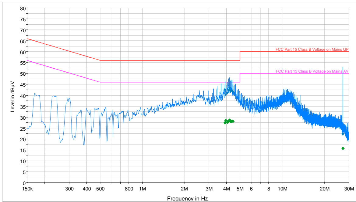
Plot 6-25. Line-Conducted Test Plot (N)
