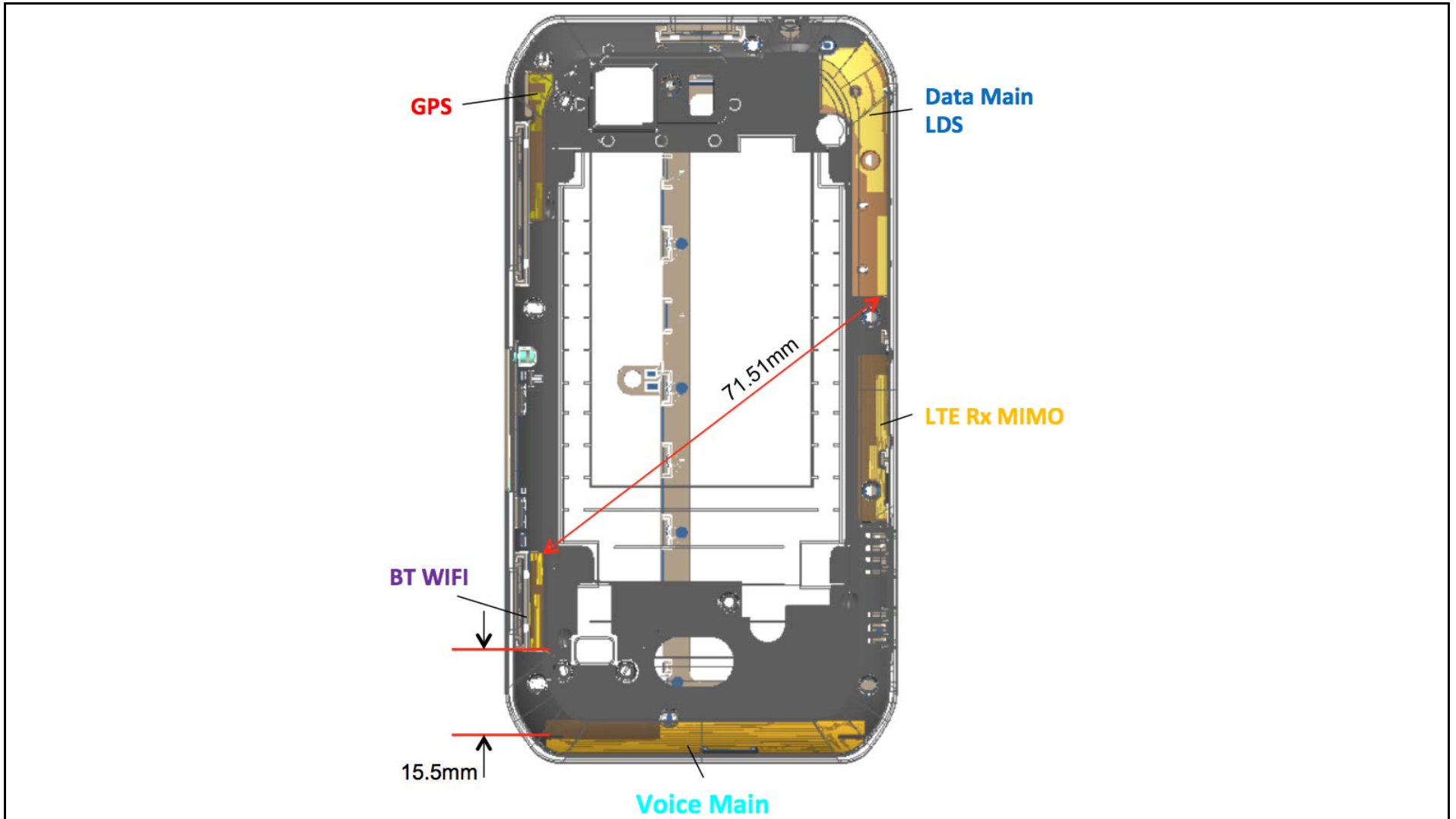
Photograph 9-7: Antenna Diagonal Spacing.
