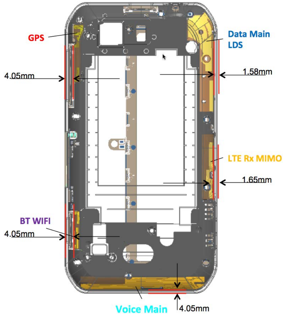
Photograph 9-6: Antenna to Phone Edge Spacing.
