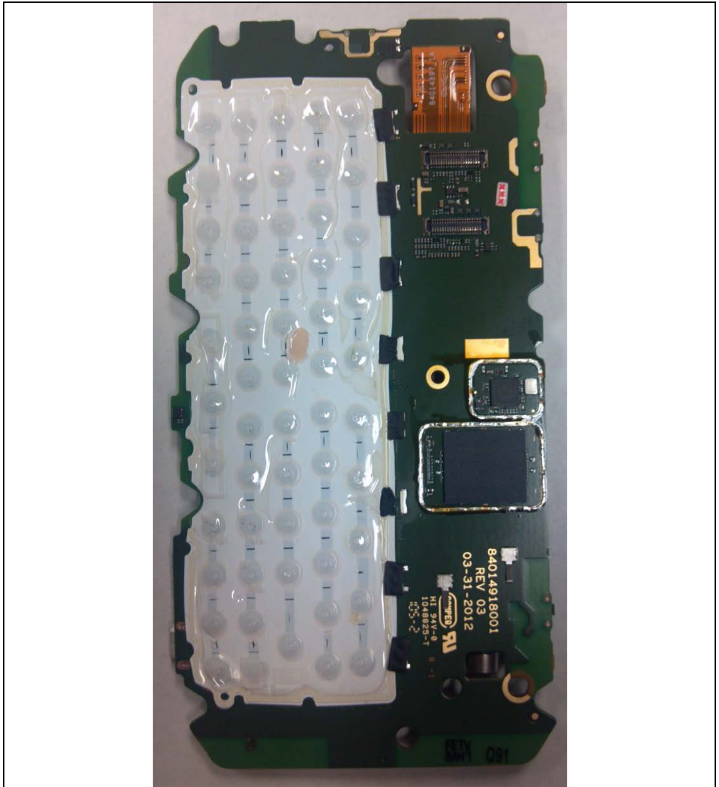
Photograph 9-3: Front (Keypad) side view of the device's PC Board, Shields Removed.
