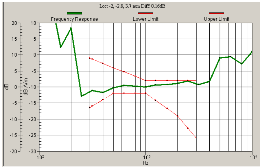
Graph 3: CDMA 1900 Frequency Response
