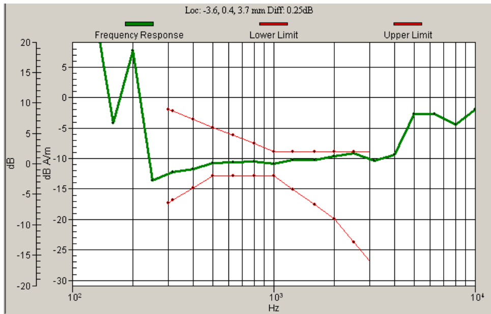
Graph 4: CDMA BC 10 Frequency Response
