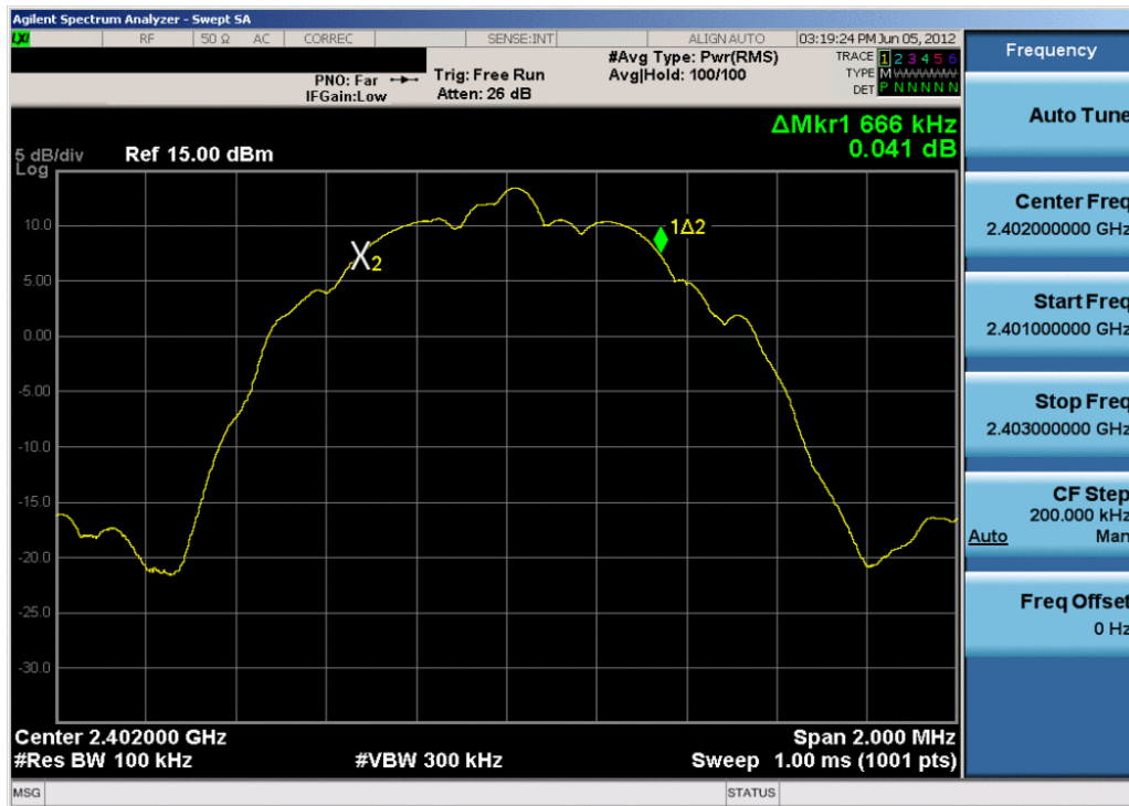
Plot 6-1. 6dB Bandwidth Plot (Bluetooth (LE) – Ch. 0)
