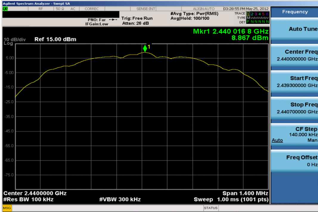
Plot 6-5. Power Spectral Density Plot (Bluetooth (LE) – Ch. 19)
