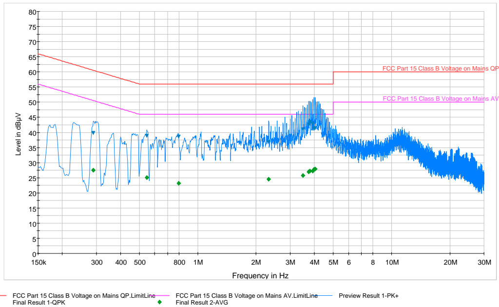
Plot 6-31. Line Conducted Plot with 802.11a (L1)
