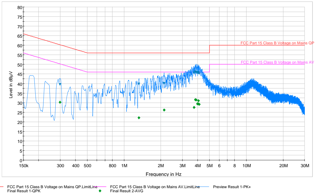
Plot 6-17. Line Conducted Plot with Bluetooth LE (N)
