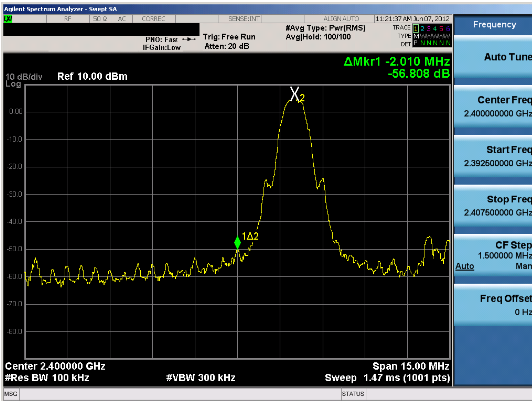
Plot 6-8. Band Edge Plot (Bluetooth (LE) – Ch. 0)
