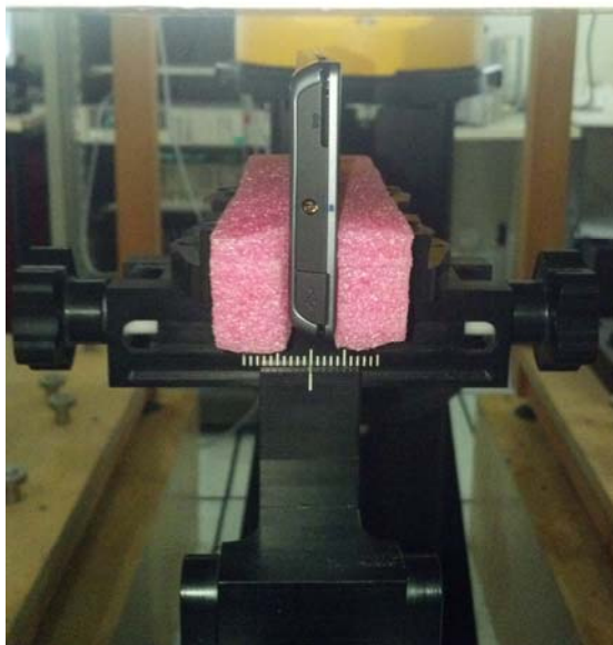
Figure 6: Mobile Hotspot Position, Long Edge (Left / Right) of Phone facing Phantom (10 mm separation)
