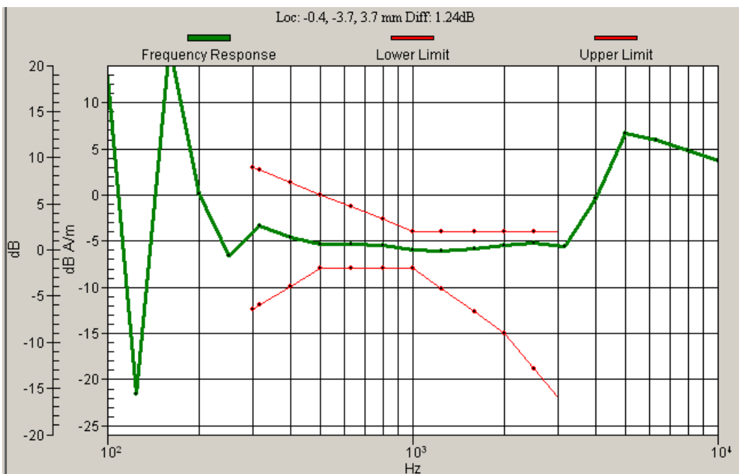
Graph 4: WCDMA 1700 Frequency Response
