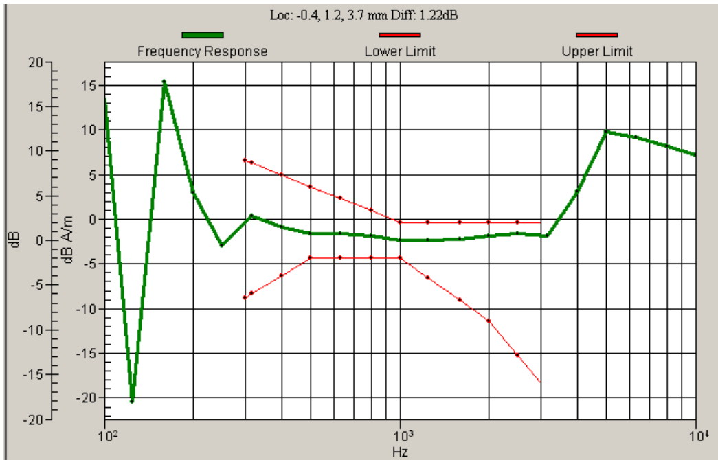
Graph 3: WCDMA 850 Frequency Response
