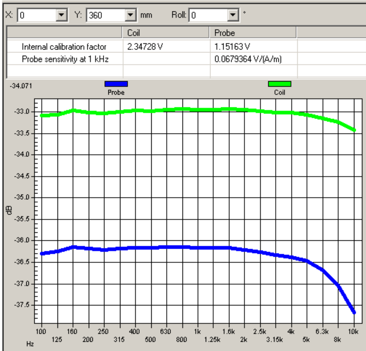
Graph 1: Frequency Response measured in AMCC
