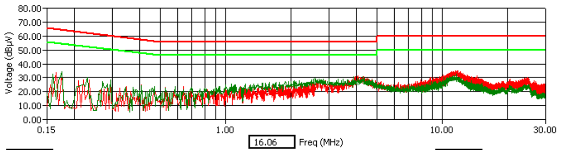
High Channel - Tx Mode - AVG Detector
