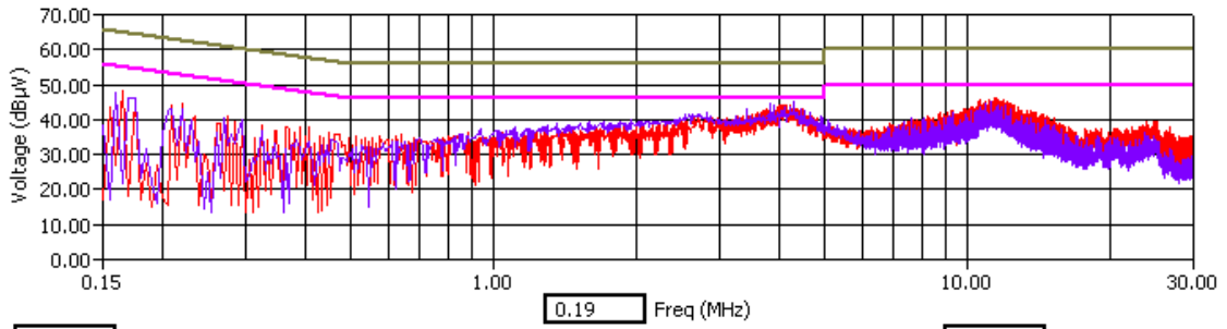
High Channel - Tx Mode - Peak Detector
