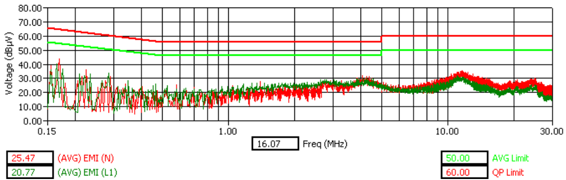
Bluetooth – Hopping - Tx Mode – AVG Detector
