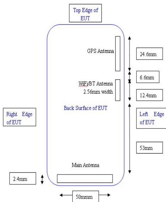
Figure 2: Antenna Separation Distances
