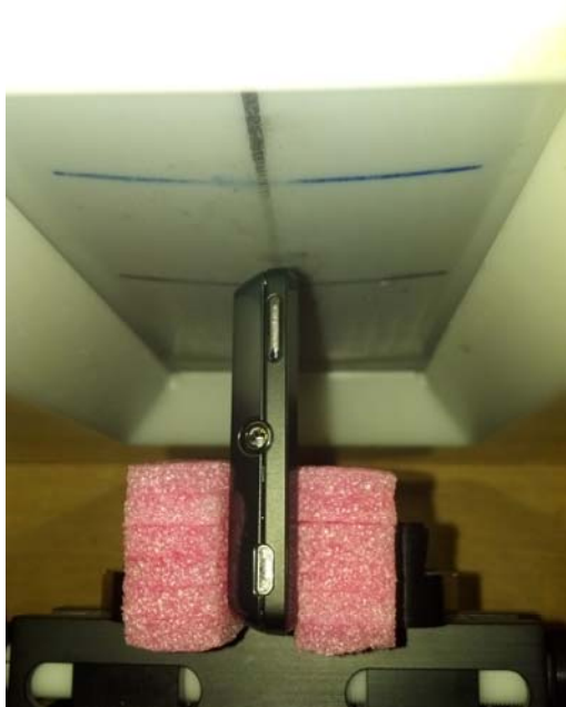
Figure 9: Mobile Hotspot Position, Right Edge of Phone facing Phantom (10 mm separation)
