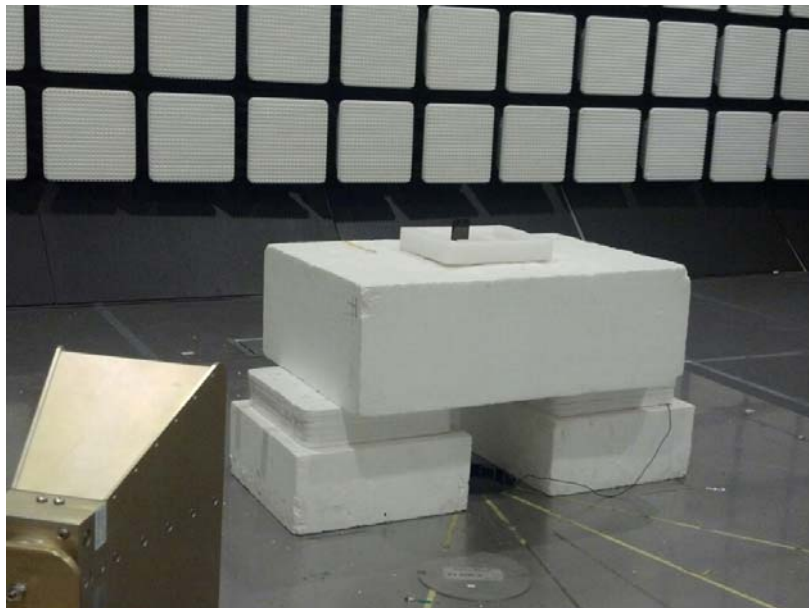
Radiated Emissions 3GHz – 18GHz
