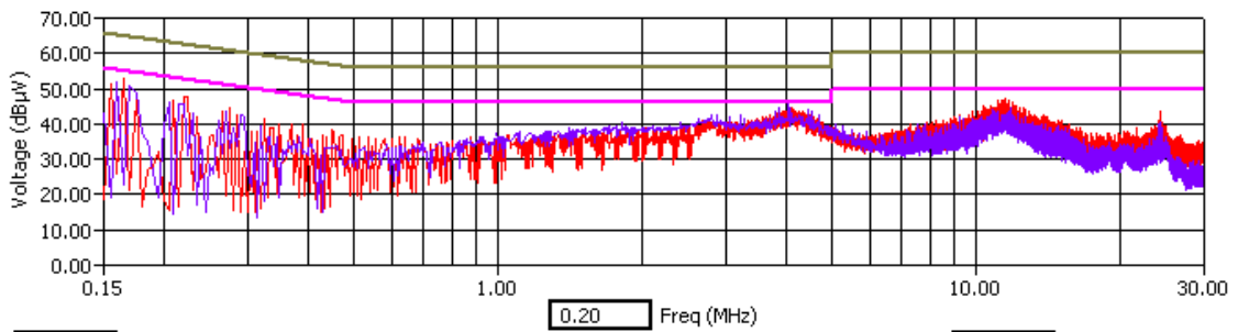
Low Channel - Tx Mode – Peak Detector
