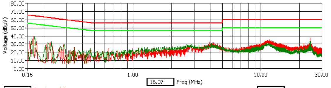
Low Channel - Tx Mode – AVG Detector
