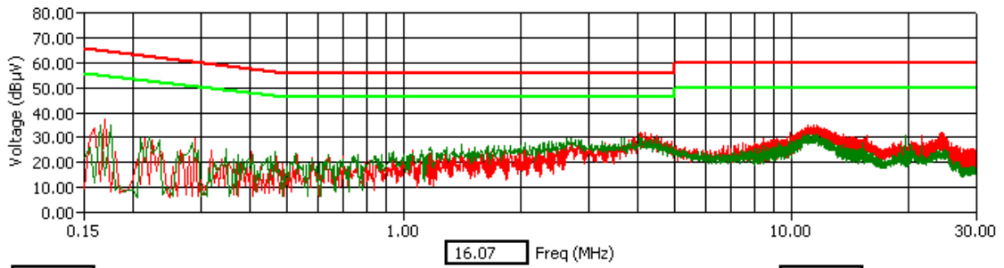
Mid Channel - Tx Mode - AVG Detector
