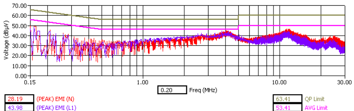
WLAN Channel 11 - Tx Mode - Peak Detector
