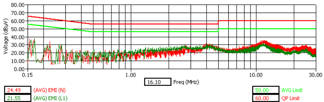
WLAN Channel 11 - Tx Mode - AVG Detector
