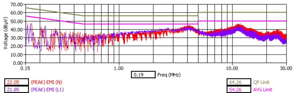
WLAN Channel 1 - Tx Mode – Peak Detector
