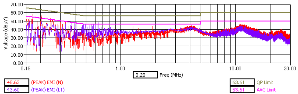
WLAN Channel 6 - Tx Mode - Peak Detector
