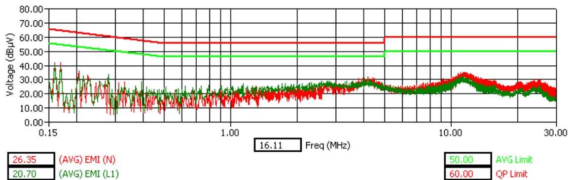
WLAN Channel 6 - Tx Mode - AVG Detector
