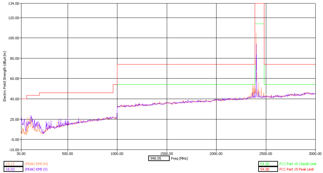
30 MHz – 3 GHz Low Channel Dual Polarization X
