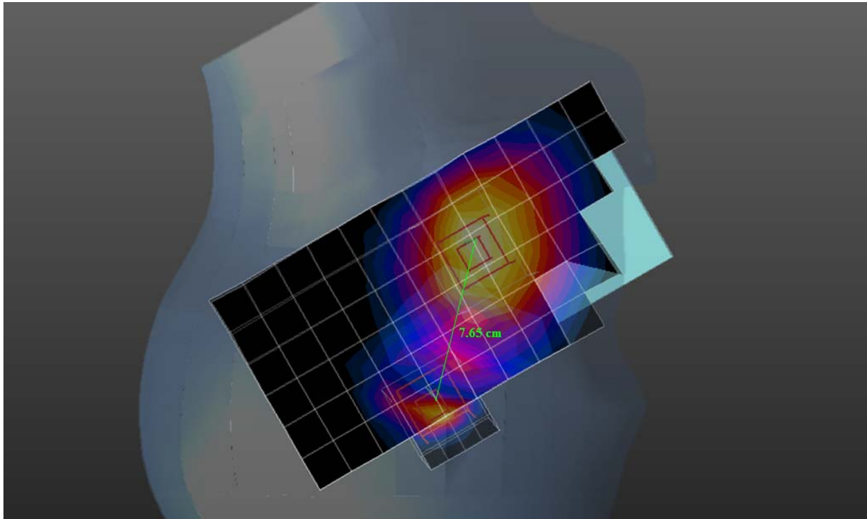
WCDMA 850 Right Head Cheek SAR overlaid with Wi-Fi 2.4 GHz Right Head Cheek SAR
