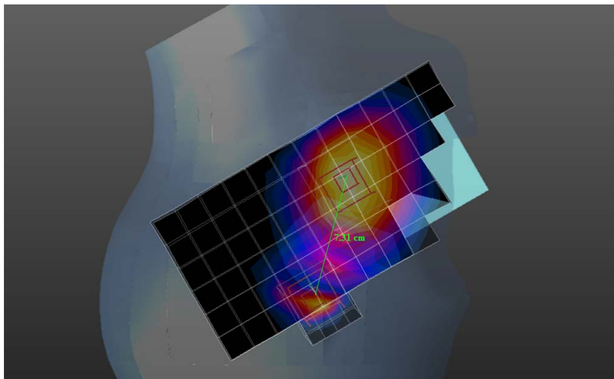
GSM 850 Right Head Cheek SAR overlaid with Wi-Fi 2.4 GHz Right Head Cheek SAR
