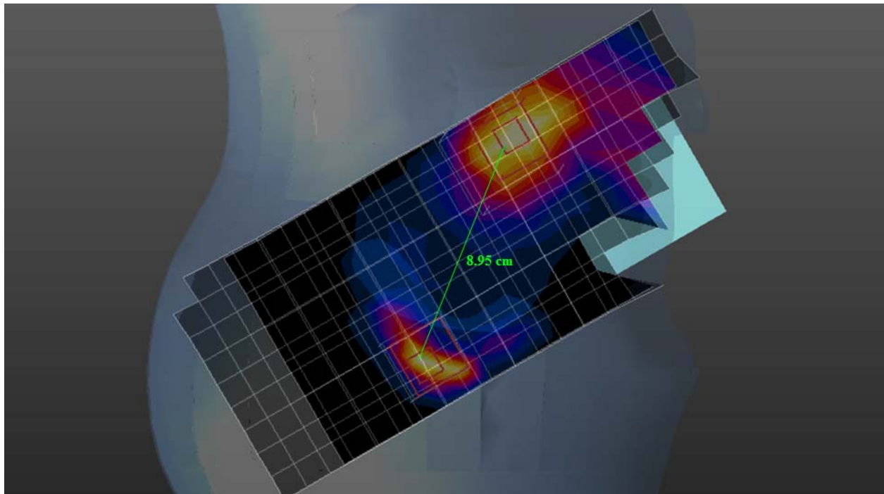
WCDMA 1900 Right Head Cheek SAR overlaid with Wi-Fi 5 GHz Right Head Cheek SAR
