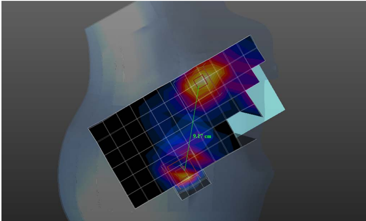
GSM 1900 Right Head Cheek SAR overlaid with Wi-Fi 2.4 GHz Right Head Cheek SAR
