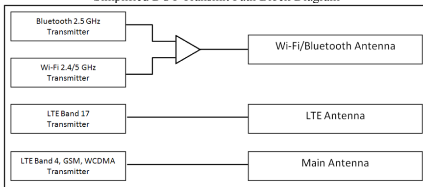
Simplified DUT Transmit Path Block Diagram
