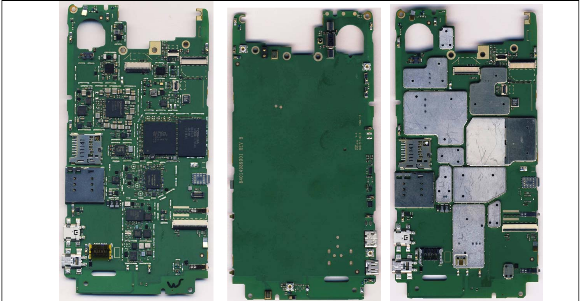
Photograph 9-2: Main PC Board, Shown with and without Shields in place (Component Side) and Non-Component Side.
