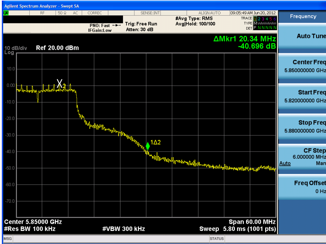
Plot 6-52. Band Edge Plot (20MHz BW 802.11n (5.8GHz) – Ch. 165)
